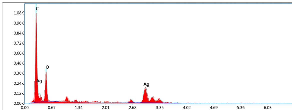
Figure 5. The EDX analysis for Ag NPs (prepared via Cynara extract, after heat treatment (amber colour)).
