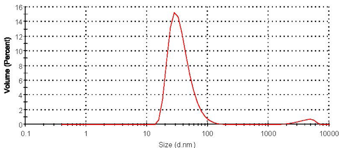
Figure 3. The PSD graph for Ag-NPs via Cynara after heat treatment (amber colour).
