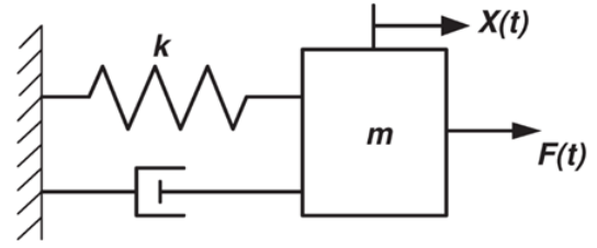
Fig. 2. A Mass- spring- damper system with external force
