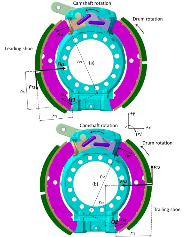
Figure 5. Forces acting on the shoes of Z-cam brake: (a) Leading side, (b) Trailing side.
