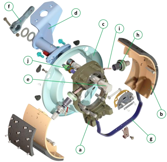
Figure 1. Z-cam drum brake components: (a) Torque plate, (b) Shoes, (c) Dust shield, (d) Bracket, (e) Shaft, (f) Lever, (g) C-spring, (h) Tappet heads, (i) Struts and (j) Parts of automatic adjustment mechanism.
