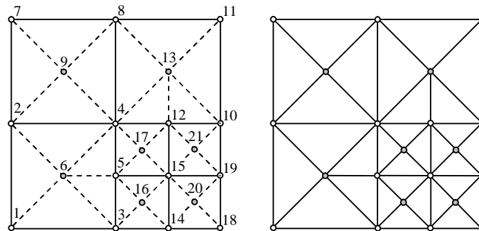
Figure 3. Node numbering and triangular mesh generated from quad-tree grid
