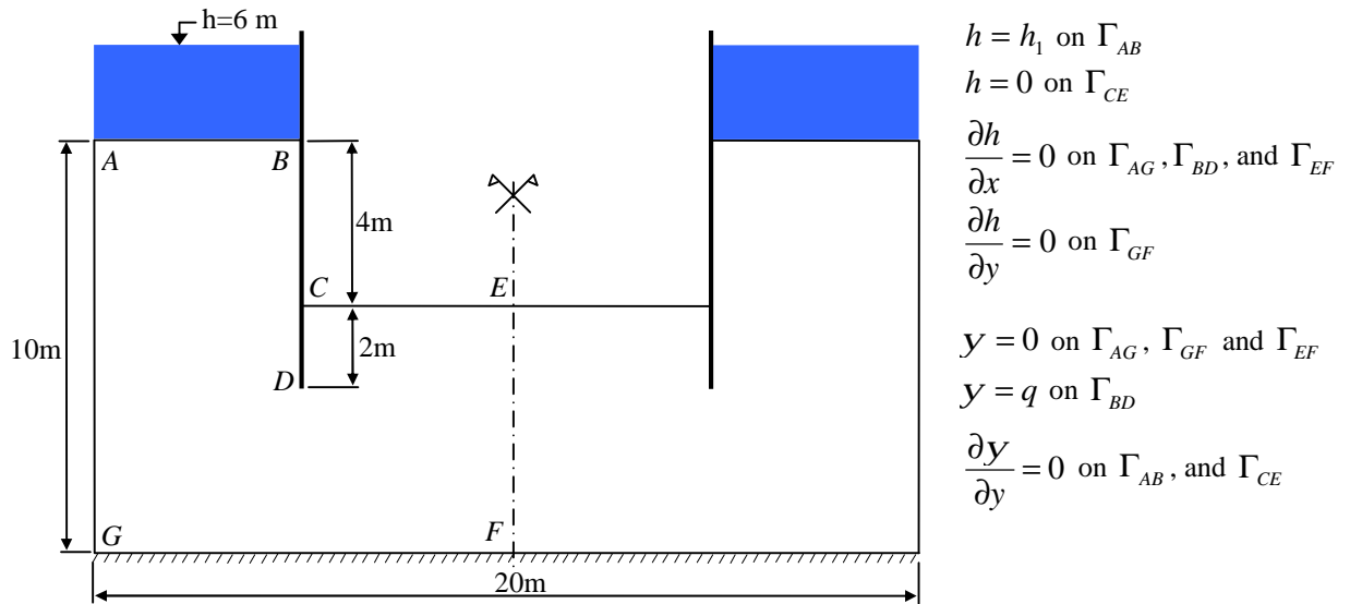
Figure 12. Problem geometry and boundary conditions
