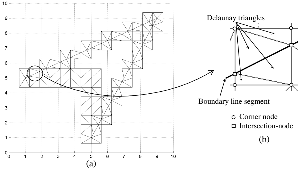
Figure 5. Test example; a) boundary line containing cells , b) nodes and Delaunay triangles for a chosen cell
