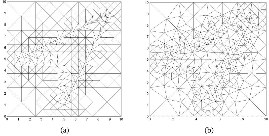
Figure 6. Test triangulation a) before and b) after Laplacian smoothing
