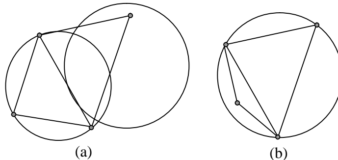
Figure 4. a) Triangulation which obeys empty circle criterion, b) triangulation which does not obey the criterion
