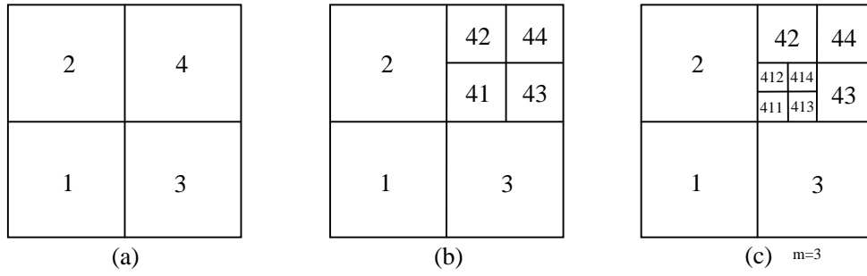
Figure 2. a) Level-one, b) level-two and c) level-three quadrants and their cell identity names
