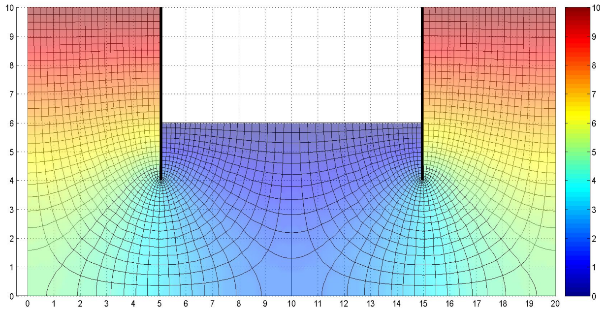
Figure 14. 2-D contour plot of function f and y
