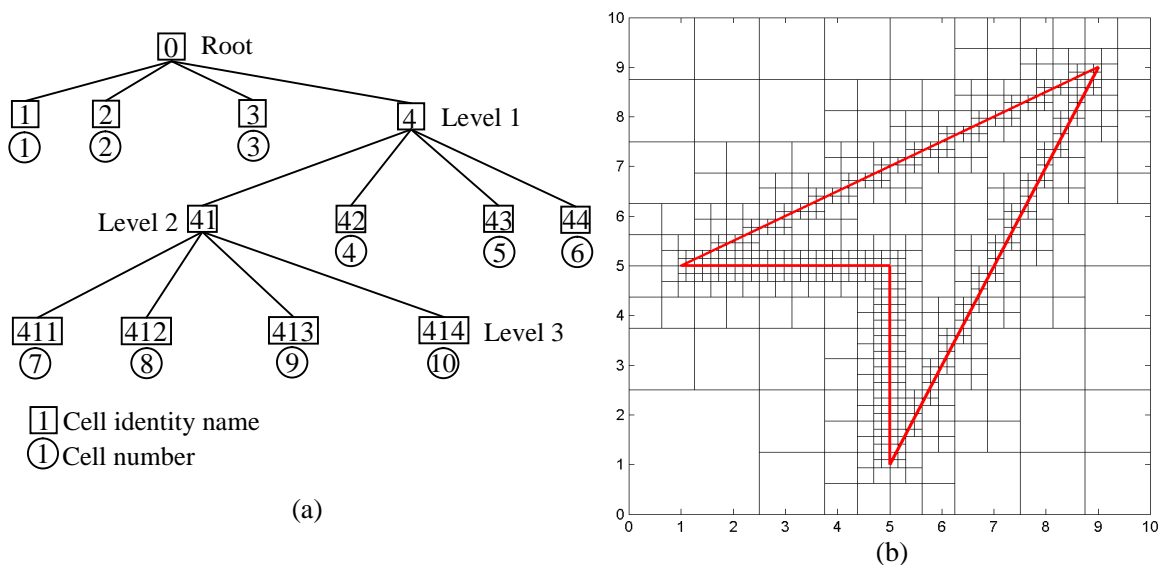
Figure 1. a) Representative quad-tree structure and b) quad-tree grid of test example
