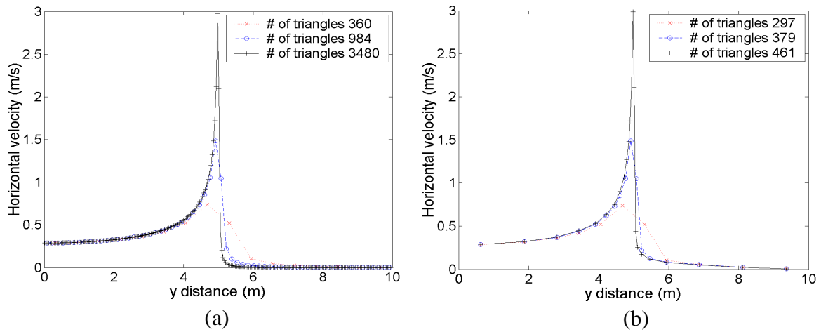
Figure 10. Horizontal component of flow velocity under the sheet pile, a) Type I mesh and b) Type II mesh
