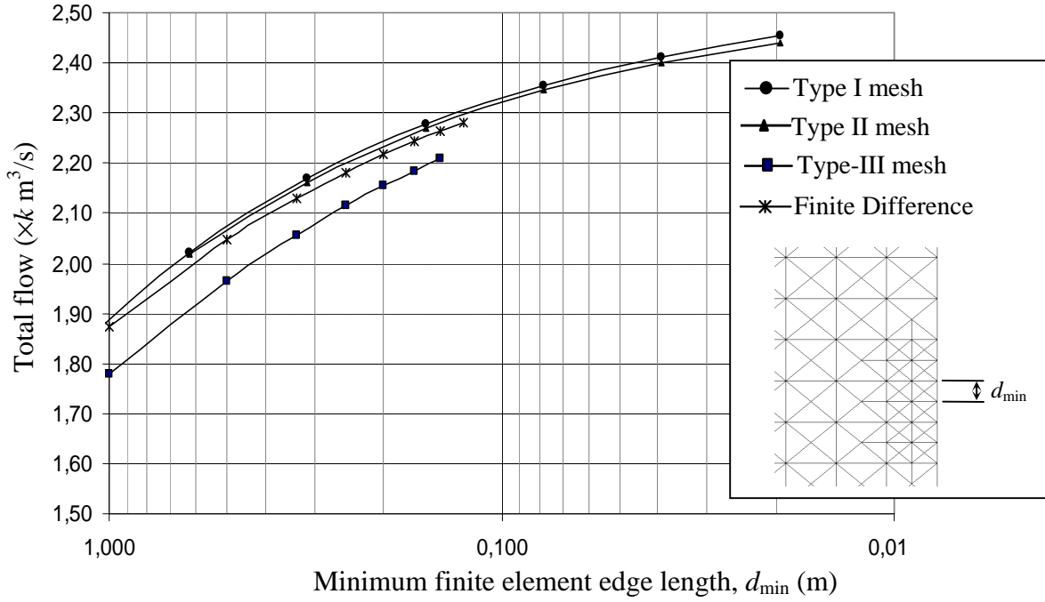
Figure 11. Change of total flow with size of element on \Gamma_{CE} boundary
