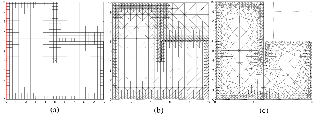
Figure 13. a) Quad-tree grid, b) triangulation based on quad-tree, c) mesh after post processing
