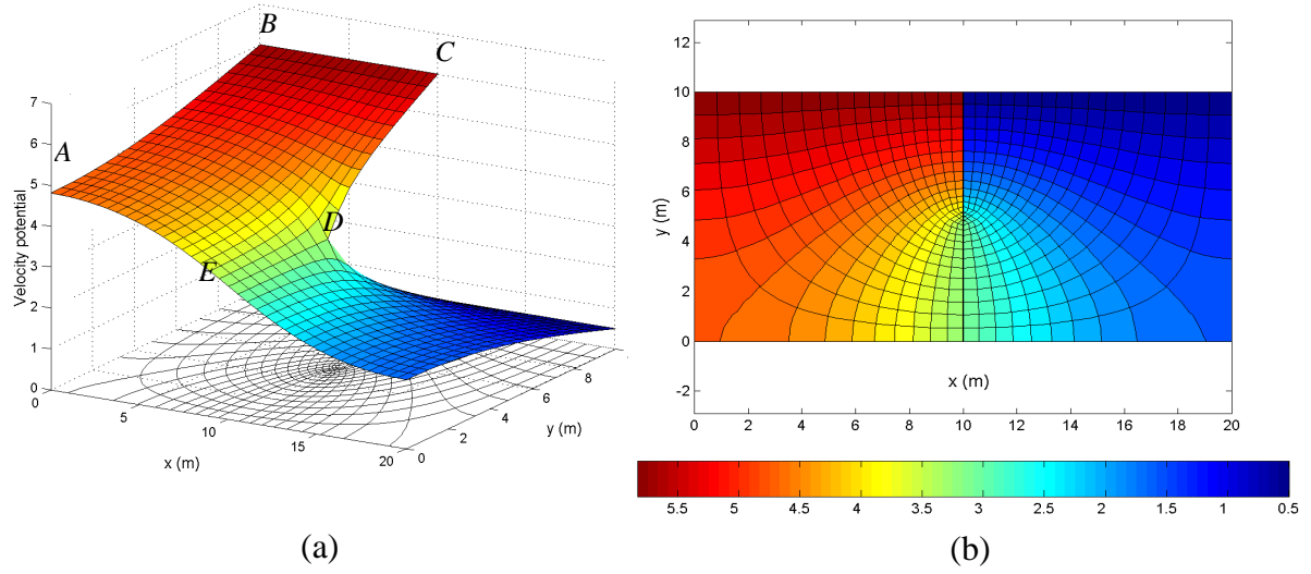
Figure 9. a) 3-D surface plot and b) 2-D contour plot of function f and y
