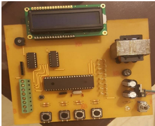
Fig. 7. Applied Circuit
