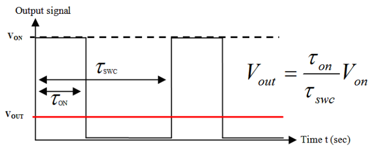
Fig. 1. Signal generation with PWM technique
