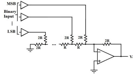
Fig. 4. R-2R Method
