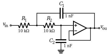
Fig. 5. Low Pass Filter values
