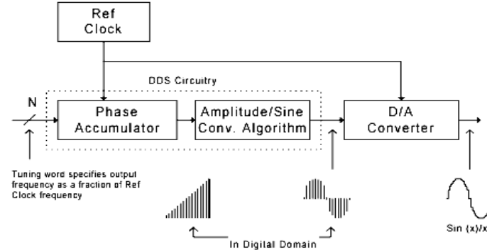
Fig. 2. Direct Digital Synthesis Method
