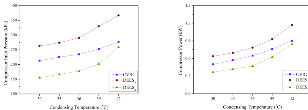
Figure 7. Variation of a) compressor inlet pressure b) compressor power depending on condensing temperature
