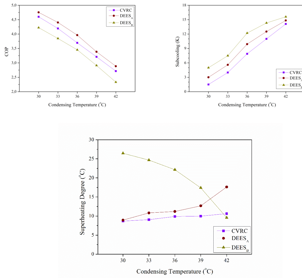
Figure 9. Variation of a) COP b) Subcooling and c) Superheat degrees depending on condensing temperature
