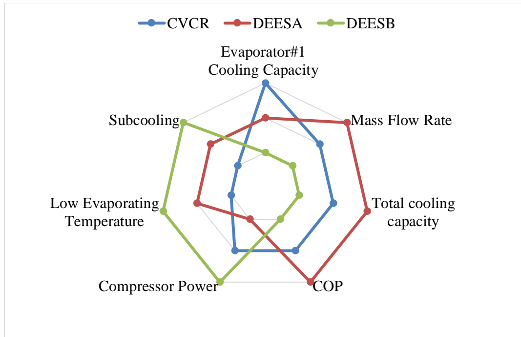
Figure 10. Comparison of DEESA, DEESB, and CVCR configurations
