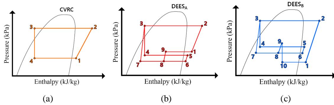
Figure 5. Pressure – enthalpy diagrams a) CVRC b) DEESA c) DEESB
