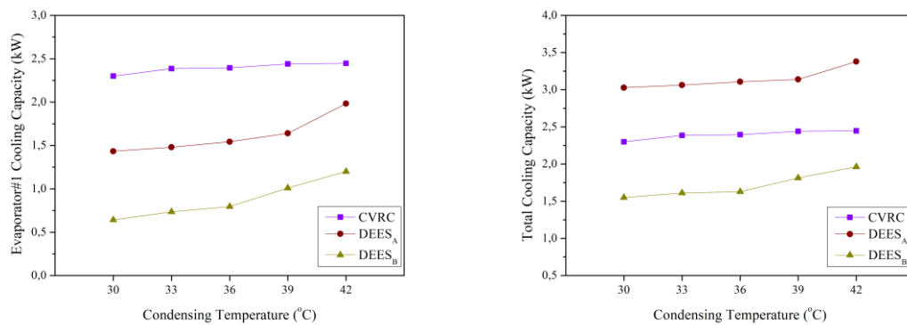
Figure 8. Variation of a) Evaporator#1 cooling capacity b) Total cooling capacity depending on condensing temperature
