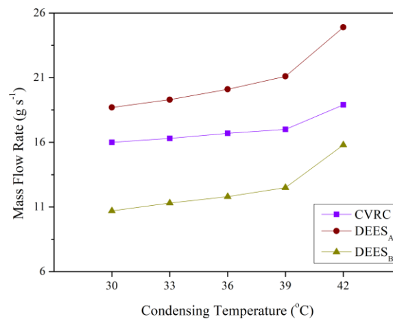
Figure 6. Variation of mass flow rate depending on condensing temperature
