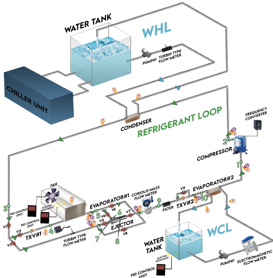
Figure 2. Schematic of experimental system
