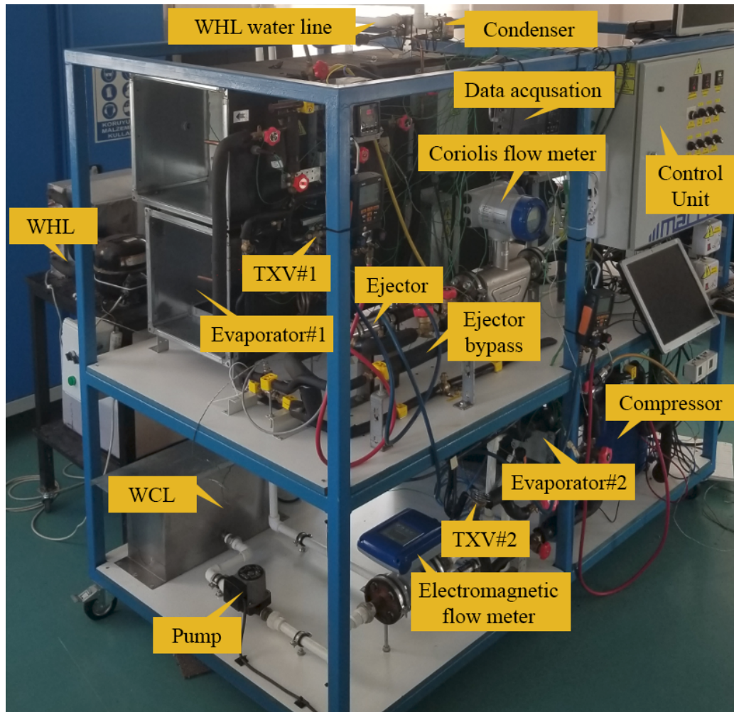
Figure 1. General view of the experimental system
