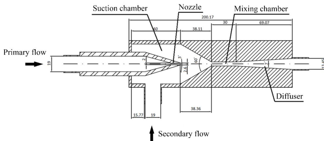
Figure 3. The ejector geometry [23]
