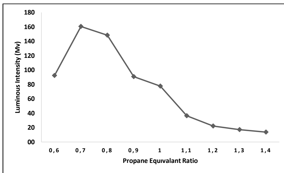
Figure 8. Luminous intensity values at different propane equivalent ratios
