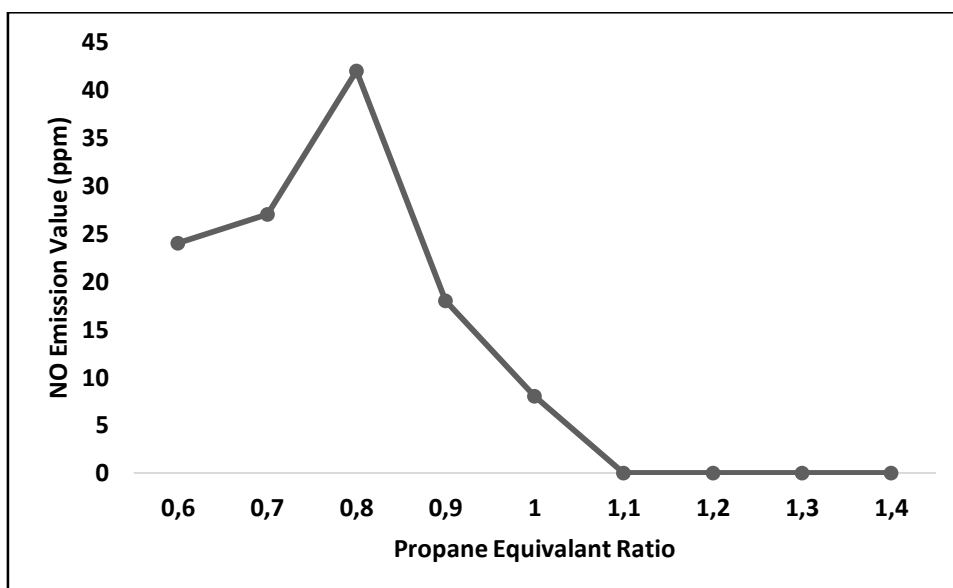
Figure 4. NO emission value at different propane equivalent ratio
