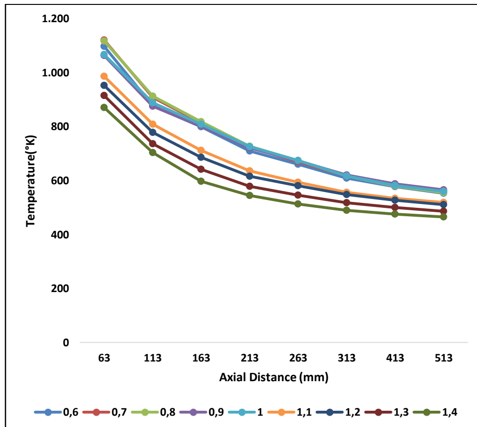
Figure 6. Axial temperature values at different propane equivalent ratios
