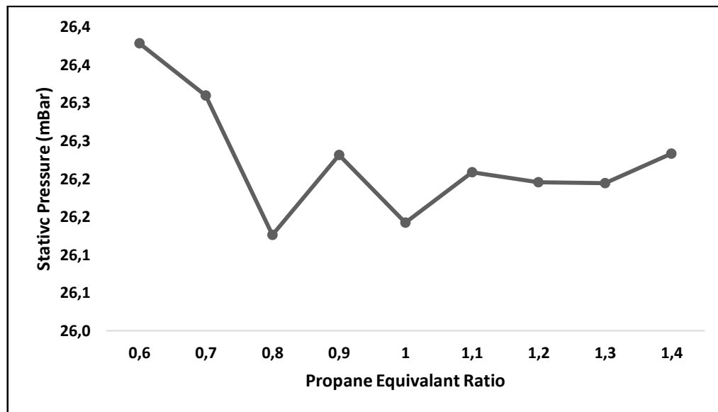
Figure 9. Static pressure values at different propane equivalent ratio
