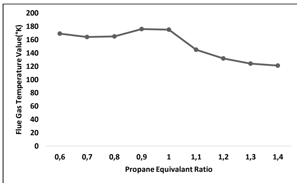
Figure 7. Flue gas temperature values at different propane equivalent ratios
