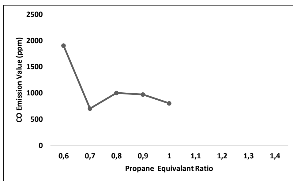
Figure 5. CO emission value at different propane equivalent ratio
