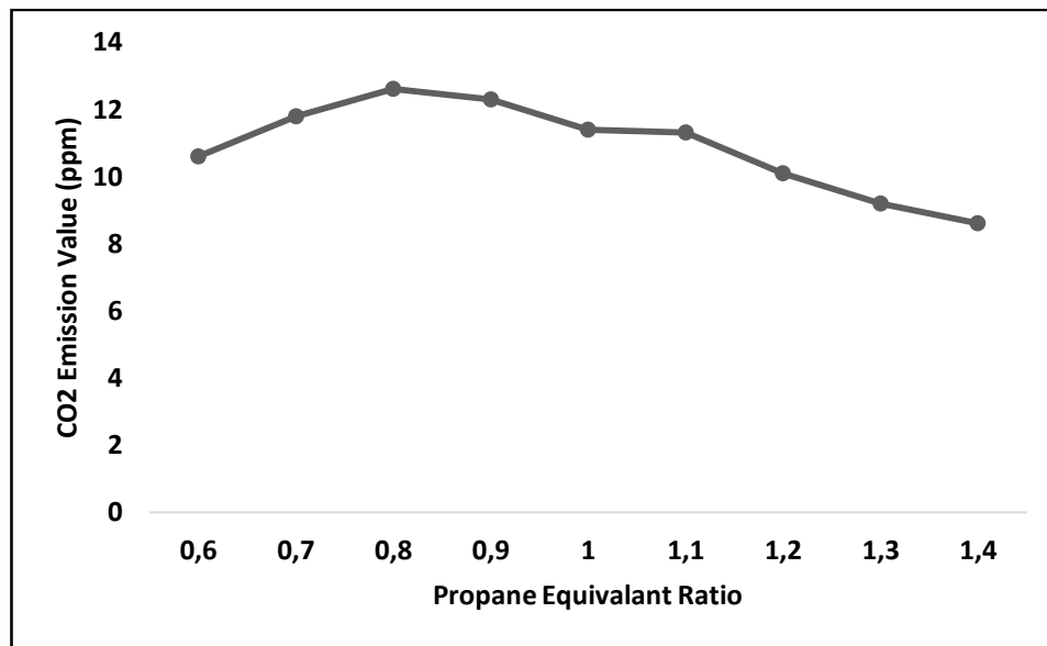
Figure 3. CO 2 emission value at different propane equivalent ratio
