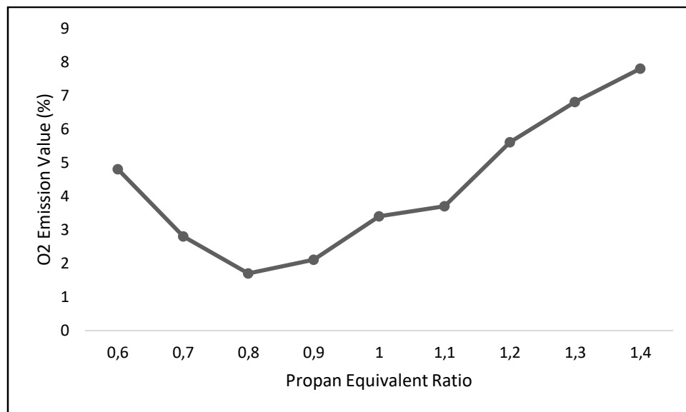
Figure 2. O 2 emission value at different propane equivalent ratio
