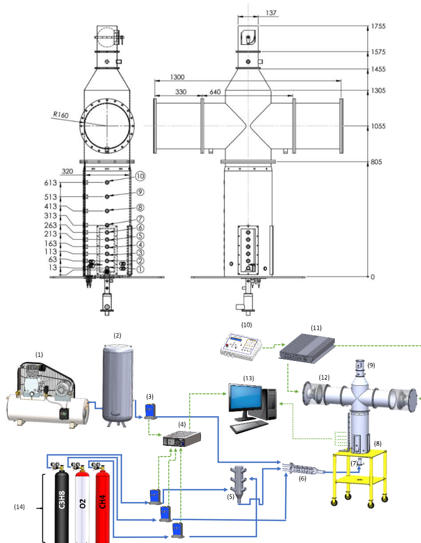
Figure 1. Experiment setup and geometric structure of the combustor (dimensions in millimeters).
