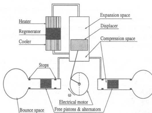
Figure 1. MARTINI-type free piston engine.
