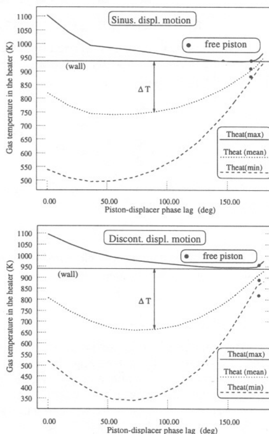
Figure 4. Temperature variations amplitude in the heater as a function of the piston-displacer phase lag.
