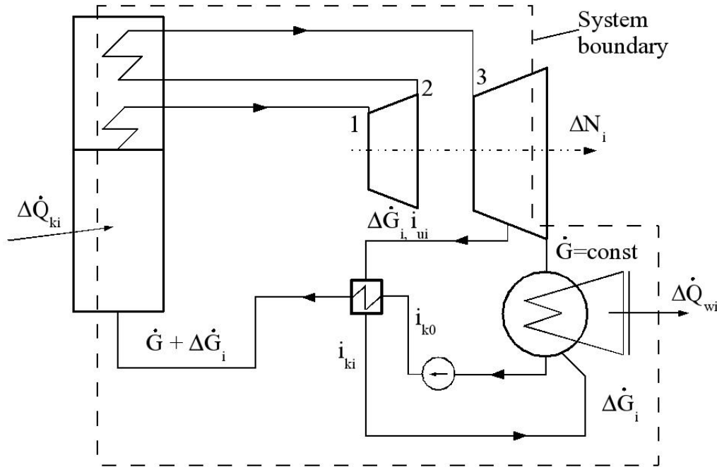
Figure 1. Scheme of steam power plant.
