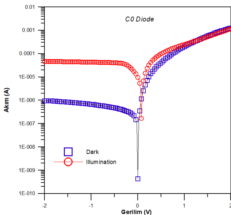
Figure 15. The semi-log I-V plots of C0 diode under dark and light (100 mW/cm 2 ).
