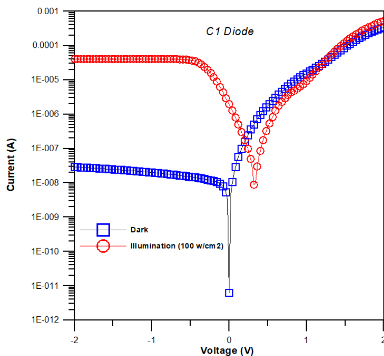
Figure 16. The semi-log I-V plots of C1 diode under dark and light (100 mW/cm 2 ).
