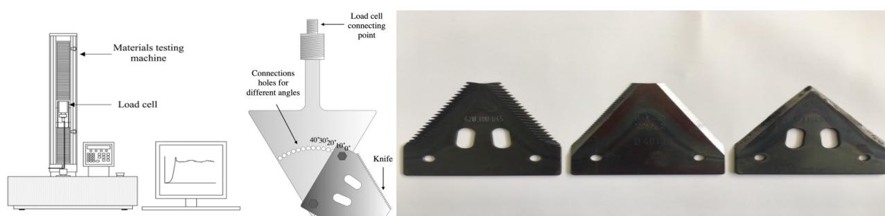
Figure 2. View of testing machine and blades
