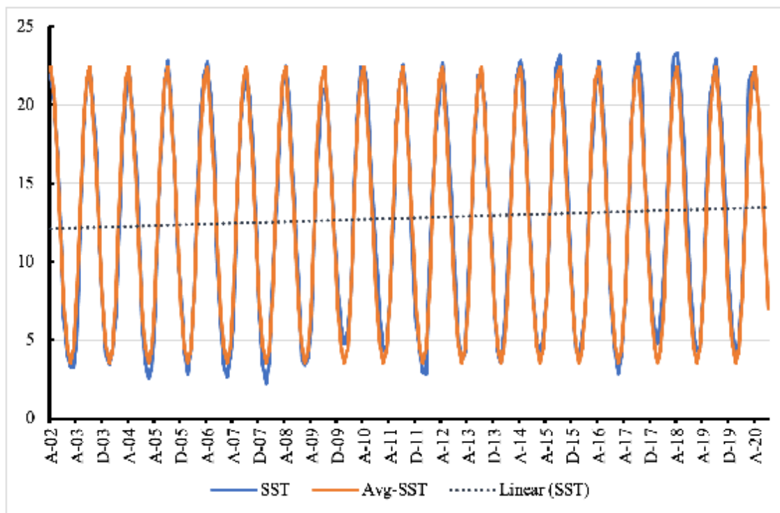
Figure 9. Long-term SST distribution with average and trendline
