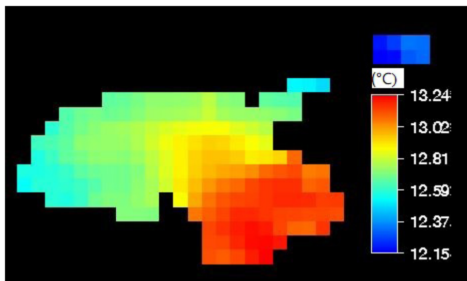
Figure 10. General average of SST of 210 images.
