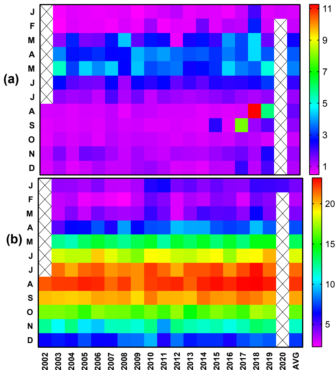
Figure 11. Monthly heatmap of Chlorophyll-a pigment concentration ( \text{mg/m}^3 ) (a) and SST ( ^{\circ}\text{C} ) (b).
