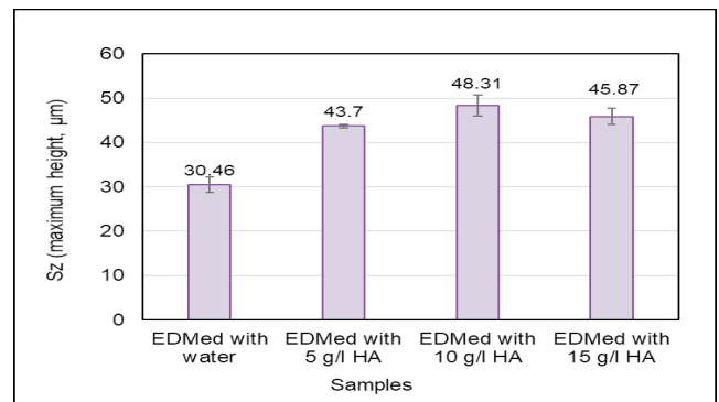
Figure 6. S_z measurement on EDM'ed and PMEDM'ed surfaces
