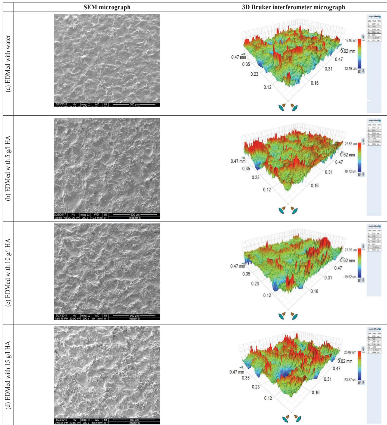
Figure 3.SEM and Bruker interferometer micrographs
