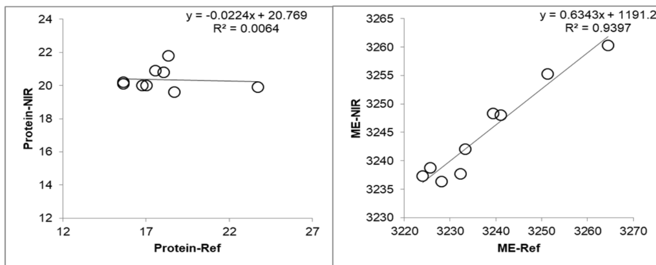
Figure 2. Regression analysis between reference analysis and NIR results of crude protein and metabolizable energy values.
