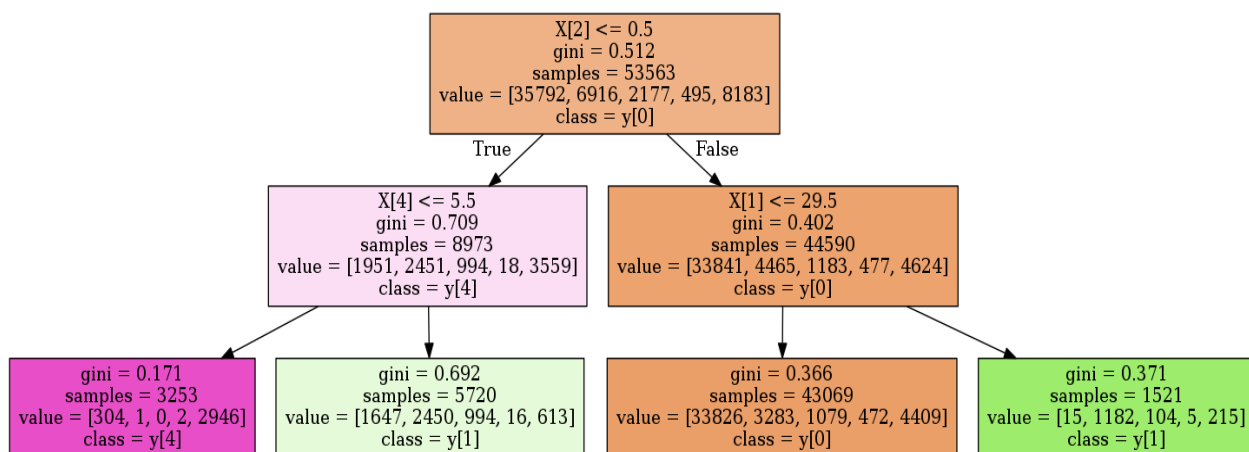
Figure 7. The schematic representation of the decision tree
