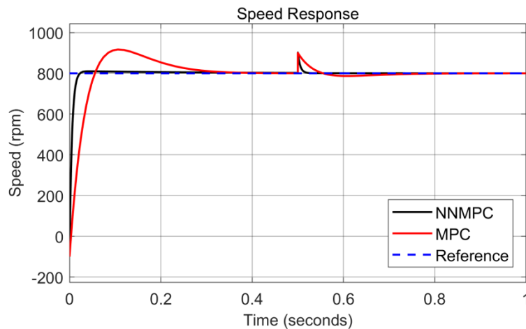
Figure 14. Speed response of the PMSM for sudden load change from 0.1 Nm to 0 Nm
