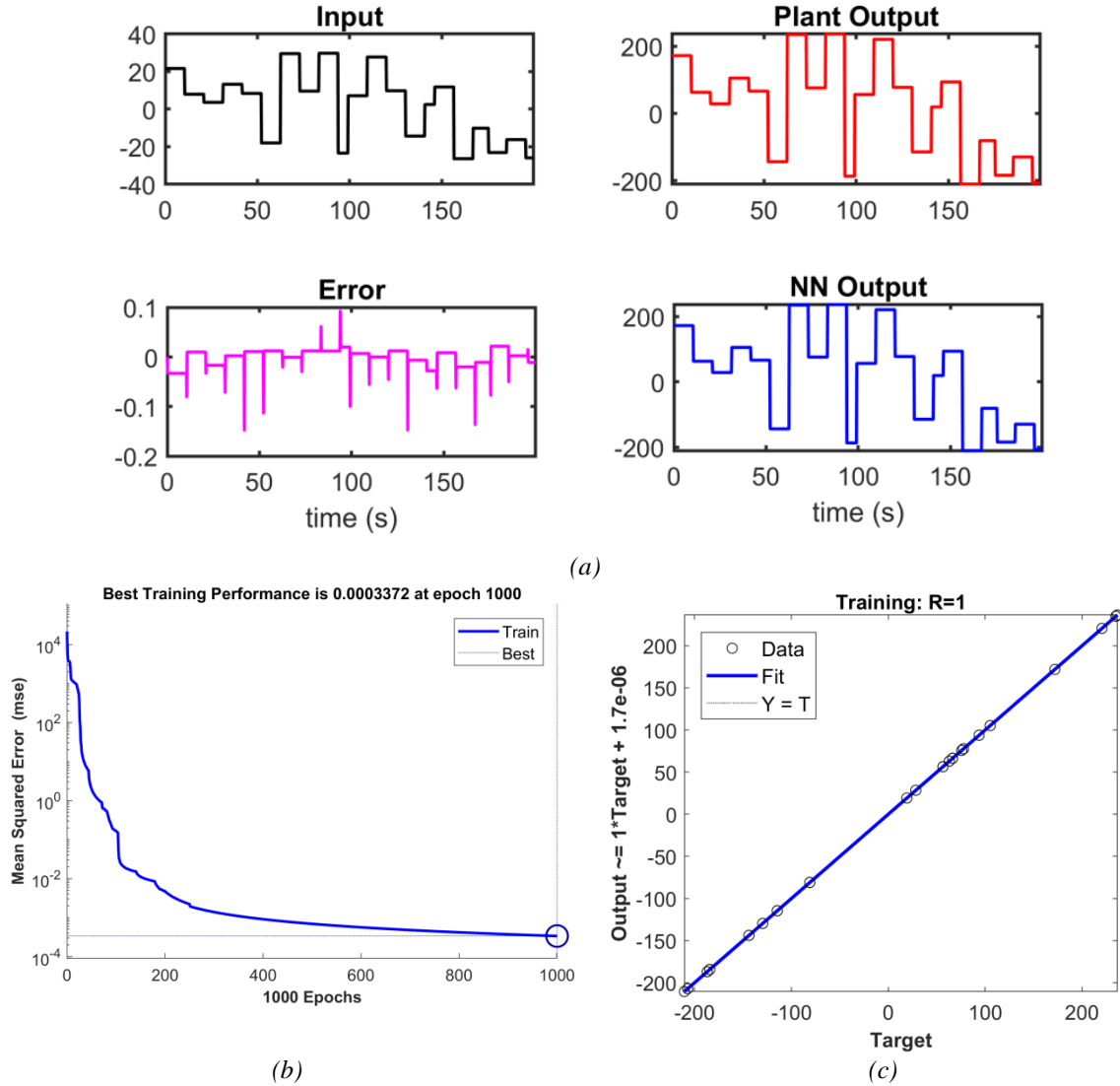
Figure 9. (a) Neural Network Model Predictive control training result (b) Performance plot (c) Regression result.
