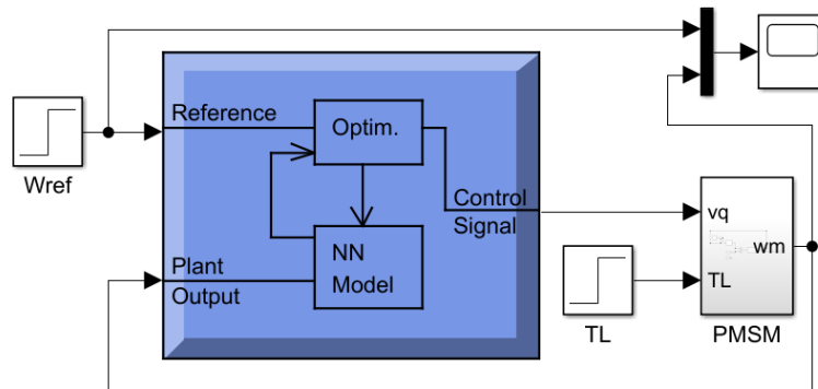
Figure 7. Simulink model of the neural network model predictive controlled PMSM
