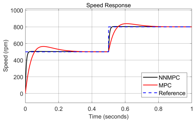
Figure 11. Speed response of the PMSM for speed reference change from 500 rpm to 800 rpm
