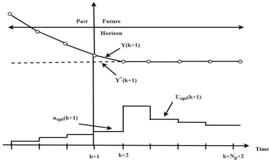
Figure 2. Prediction horizon at time step k+1
