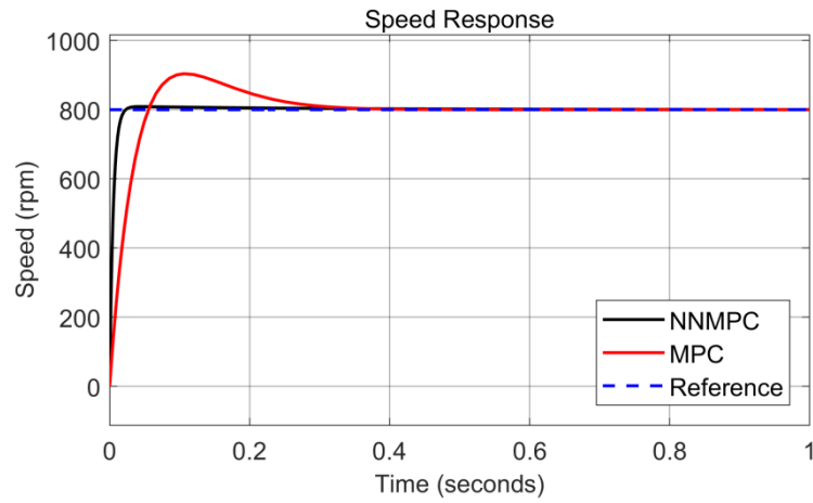
Figure 10. Speed response of the PMSM for constant set speed command
