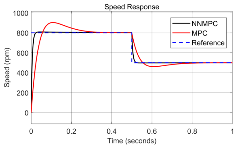
Figure 12. Speed response of the PMSM for speed reference change from 800 rpm to 500 rpm
