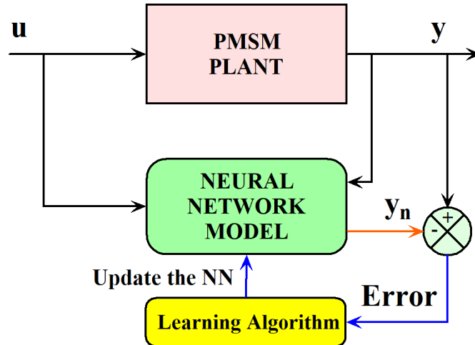
Figure 3. PMSM plant identification by neural network.
