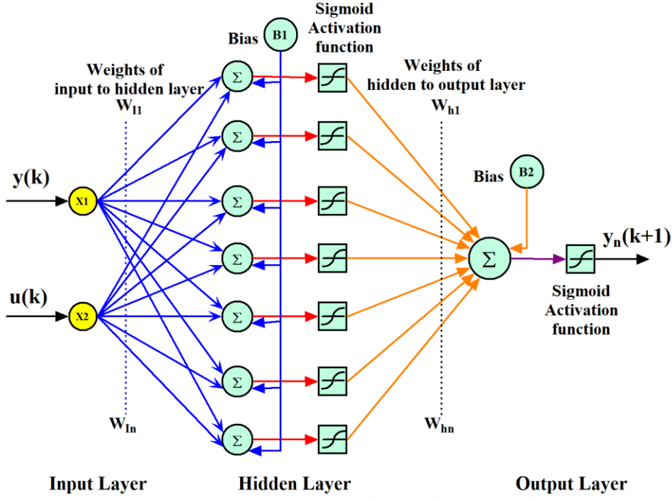
Figure 4. Structure of Neural Network Plant model
