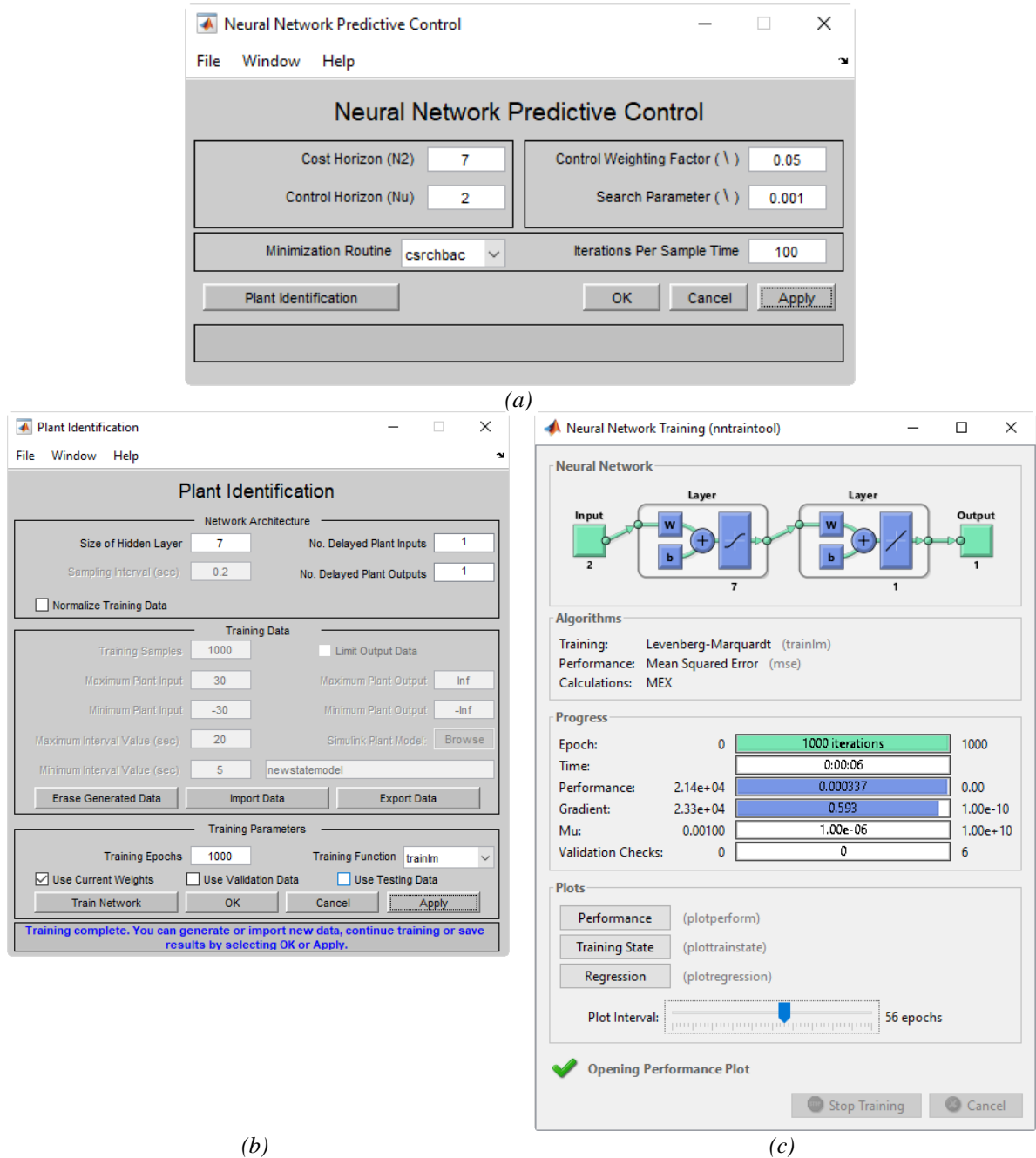
Figure 8. (a) Neural network model predictive control, (b) plant identification by NN MPC, (c) neural network training.
