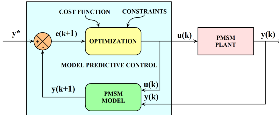
Figure 1. Model predictive controlled PMSM
