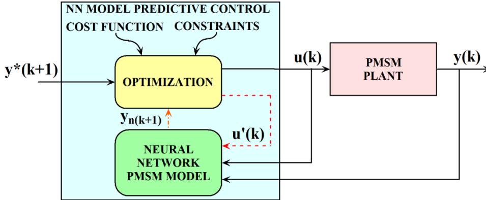
Figure 5. Neural Network Model Predictive Controlled PMSM
