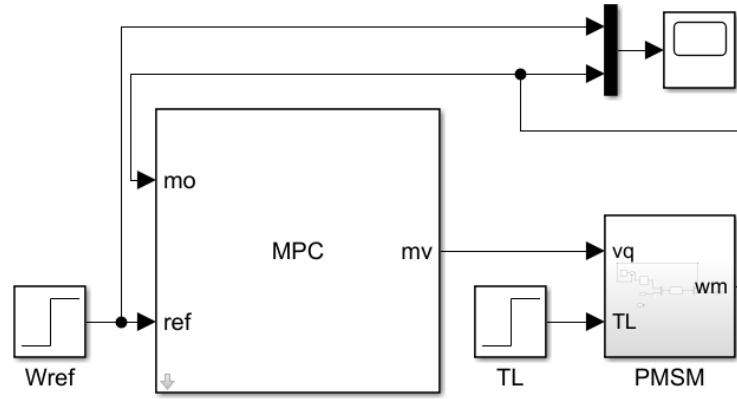
Figure 6. Simulink model of model predictive controlled PMSM
