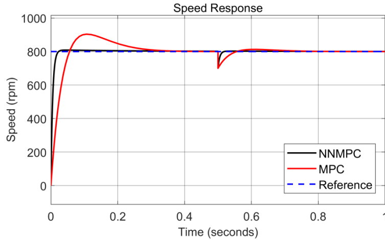
Figure 13. Speed response of the PMSM for sudden load change from 0 Nm to 0.1 Nm
