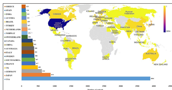
Figure 2. Global productivity world map showing the distribution of published articles about ACL by country and bar chart showing the top 20 most active countries
