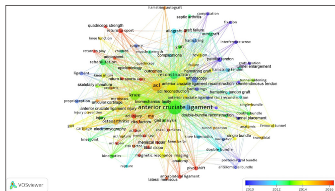
Figure 5. Network visualization map based on keyword analysis to identify past and current trends in ACL. Footnote: In the indicator given in the lower right corner of the figure, the topicality of the subject increases from blue to red (blue-green-yellow-red) over the years. The size of the circle indicates the number of uses of the keyword.
