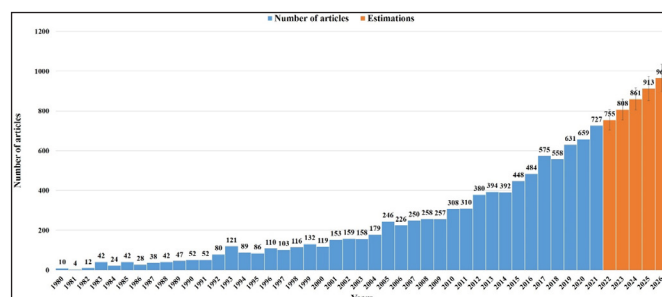
Figure 1. Bar chart showing the distribution of articles published about ACL by year and forecasts for the number of articles in the next 5 years
