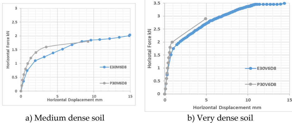
Figure 4. Verification of the finite element analysis and test results for L/D ratio of 30.
