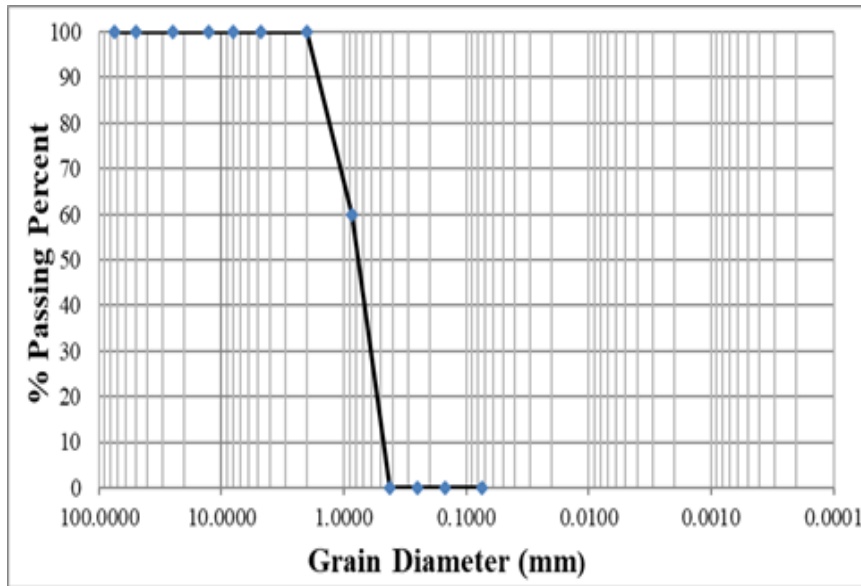
Figure 1. Grain diameter distribution of sand soil.
