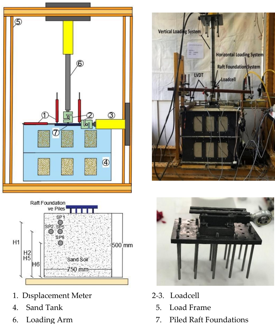
Figure 2. Experiment equipment and schematic illustration.
