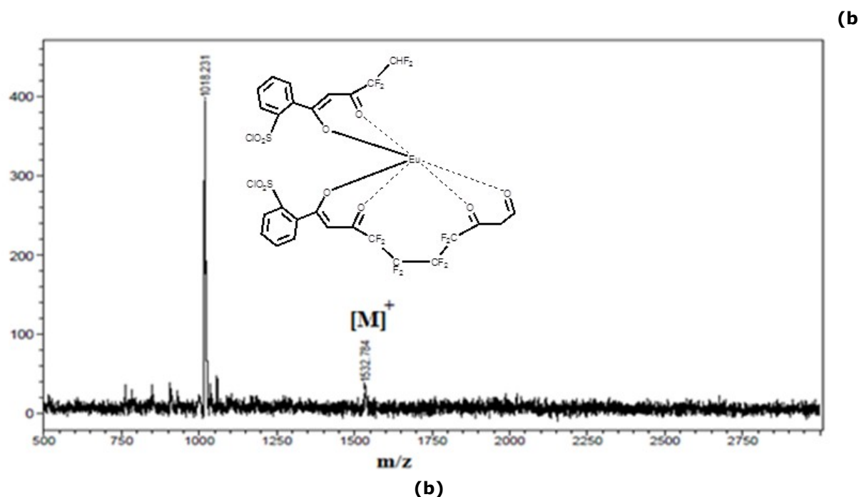
Figure 3: Mass spectra of the compounds: (a) H 2 CODIT, (b) Eu(III) chelate.
