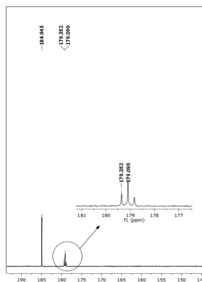
Figure 5: ^{13}\text{C} NMR spectra of the ligands: (a) \text{H}_2\text{ODIT} , (b) \text{H}_2\text{CODIT} .
