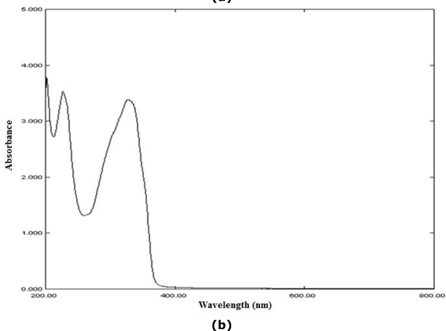
Figure 6: UV-visible spectra of (EtOH, 1.0 \times 10^{-4} M), (a) \text{H}_2\text{ODIT} , (b) \text{H}_2\text{CODIT} ligands.
