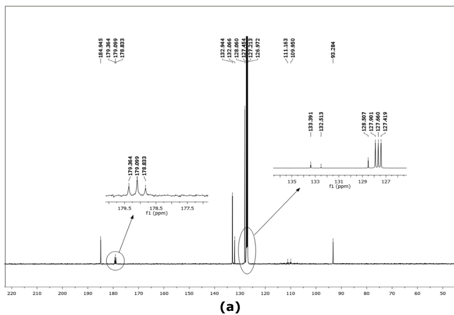
Figure 5: ^{13}\text{C} NMR spectra of the ligands: (a) \text{H}_2\text{ODIT} , (b) \text{H}_2\text{CODIT} .
