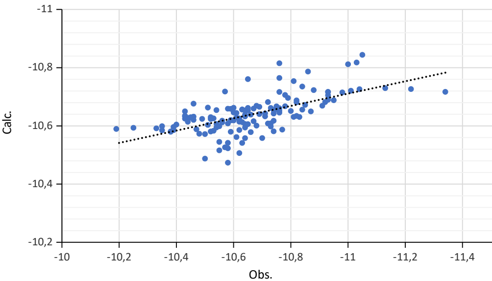
Figure 3: Graph of molecular descriptor versus independent variable importance
