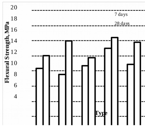
Figure 5: Flexural strength of specimens.
