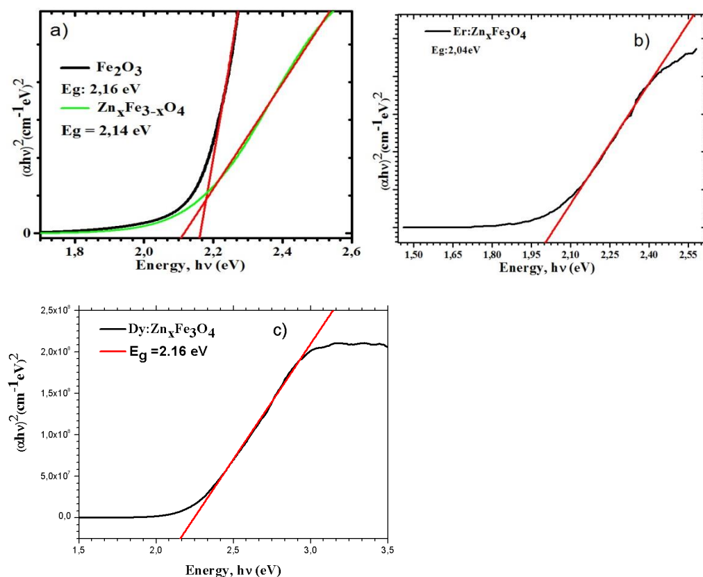
Fig.3. Plot of (\alpha h\nu)^2 (\text{cm}^{-1} \text{eV})^2 versus photon energy h\nu of a) \text{Fe}_2\text{O}_3 , \text{Zn}_x\text{Fe}_{3-x}\text{O}_4 b) \text{Er: Zn}_x\text{Fe}_{3-x}\text{O}_4 and c) \text{Dy: Zn}_x\text{Fe}_{3-x}\text{O}_4 thin films
