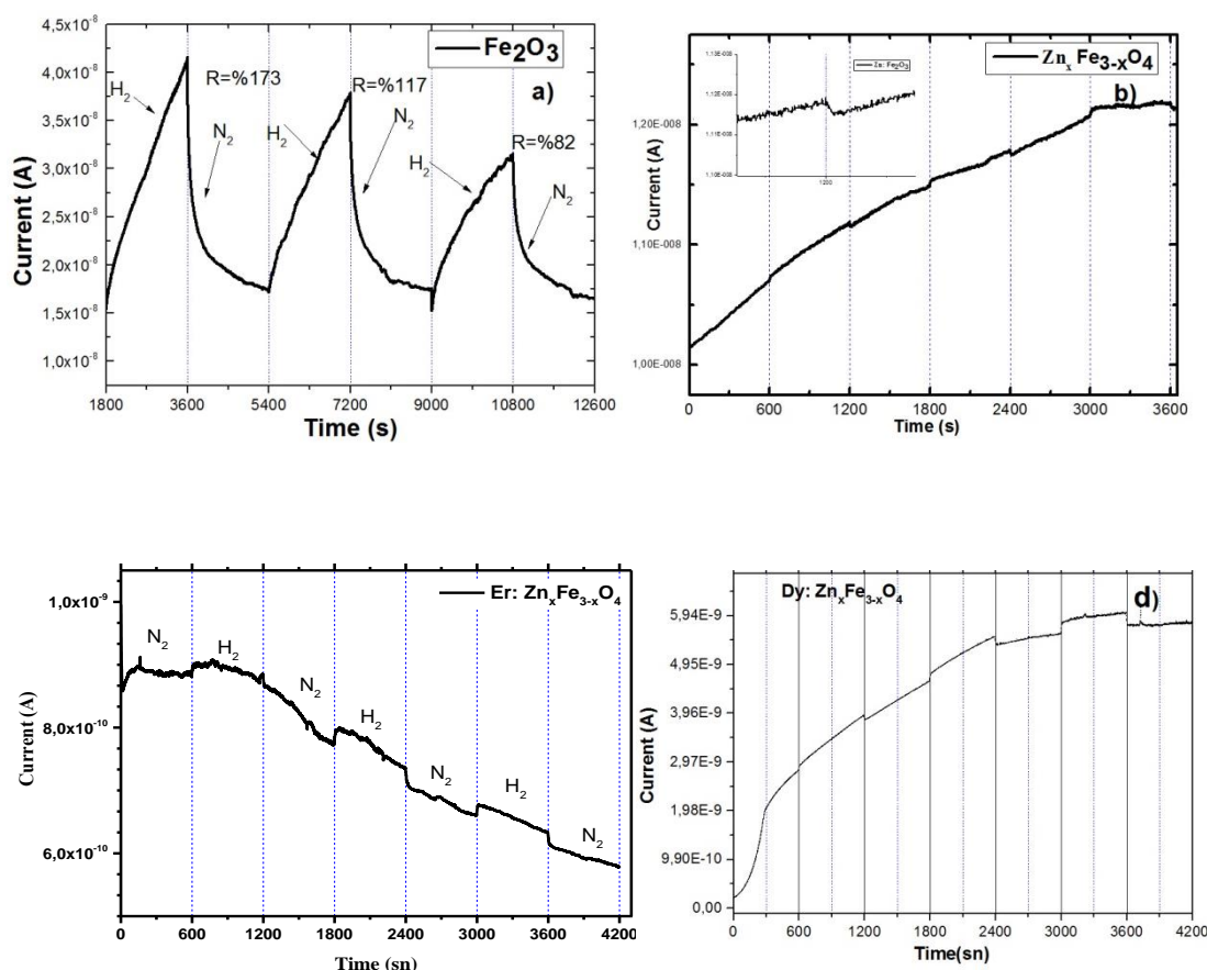
Fig. 5. Sensor Response of a) Fe 2 O 3 , b) Zn x Fe 3-x O 4 , c)Er: Zn x Fe 3-x O 4 and d) Dy: Zn x Fe 3-x O 4 thin films
