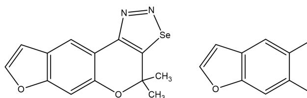
Scheme 1. 1,2,3-selendizole structure
