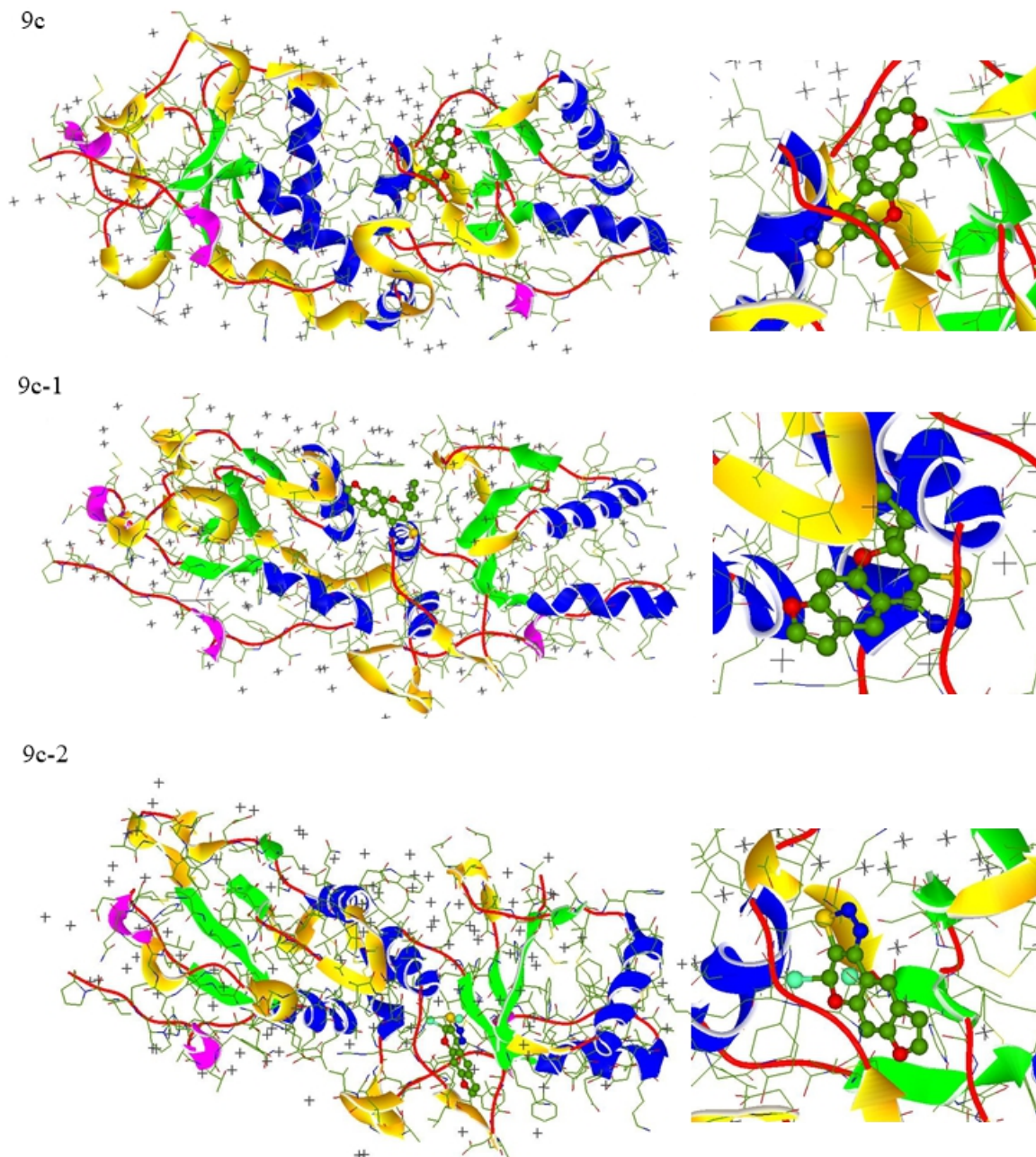
Figure 4. Binding poses of 1,2,3-selenediazole derivatives and 1JNX target protein.
