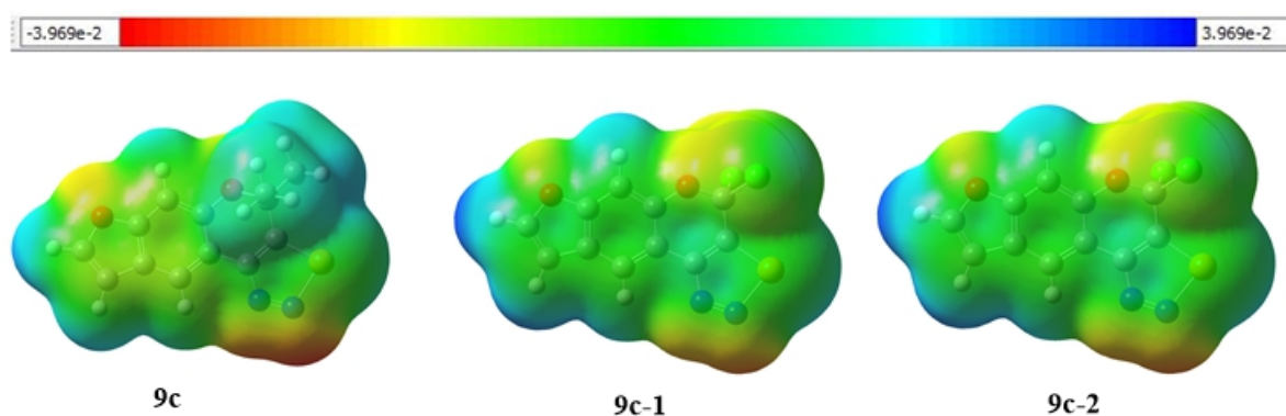
Figure 3. MEP maps of investigated 1,2,3-selendiazole derivatives
