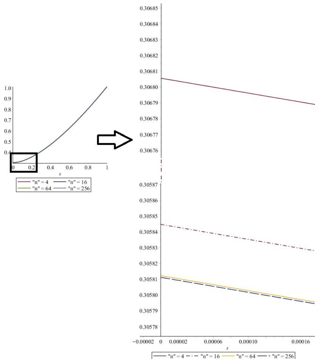
Figure 1: Comparison graphs of the approximate solutions as n increases
