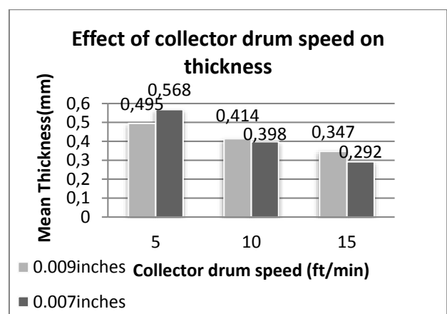
Figure 6. Change of thickness with collector drum speed
