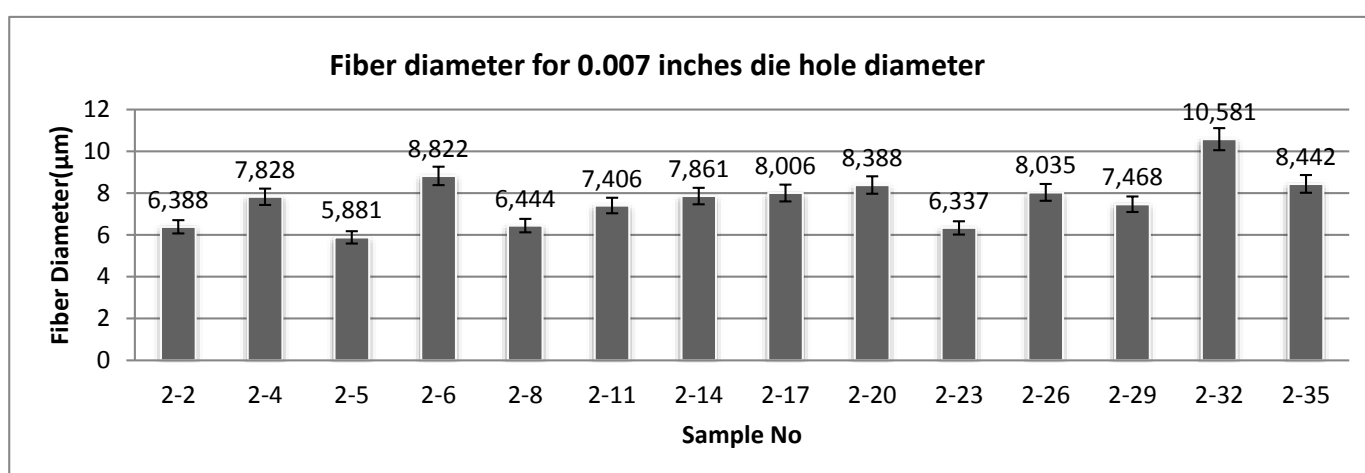
Figure 19. Fibre diameter for 0.007 inches die hole diameter
