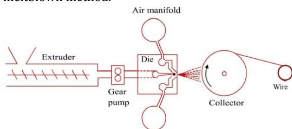
Figure 1. Schematic representation of the meltblown method[15]
