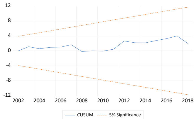
Figure 2. CUSUM Chart
