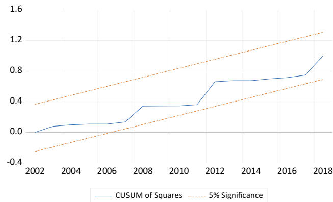
Figure 3. CUSUMQ Chart
