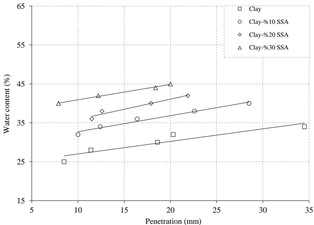
Fig 3. Variation of cone penetration with water content for clay with various SSA content
