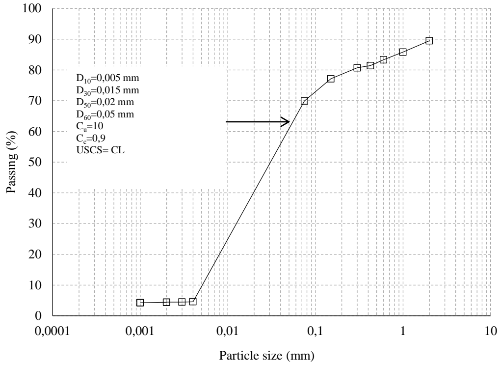
Fig 2. Particle size distributions for the clay used the experimental study
