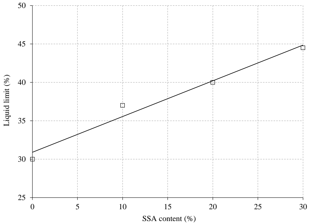
Fig 4. Liquid limit of clay with various SSA content
