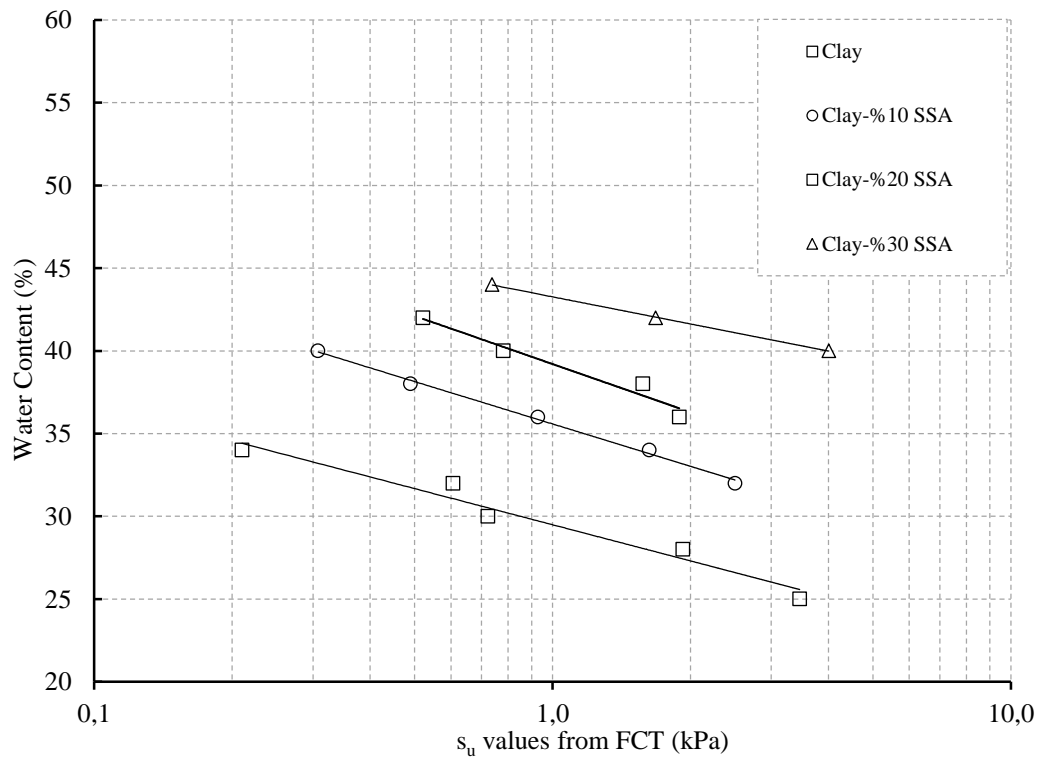
Fig 5. Relationship between undrained shear strength and water content for the clay with various SSA content
