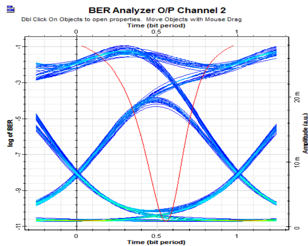
Figure 5. illustrates the log of BER vs. Time vs. Amplitude for the output of the second signal, @VCSEL, WDM, RZ, 10Gb/s, and 25Km SSF.
