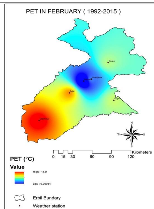
Figure 6. PET map of February
