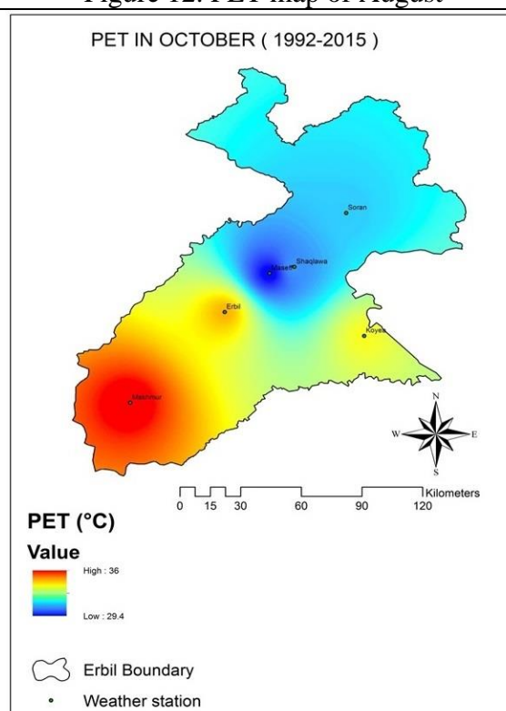
Figure 14. PET map of October
