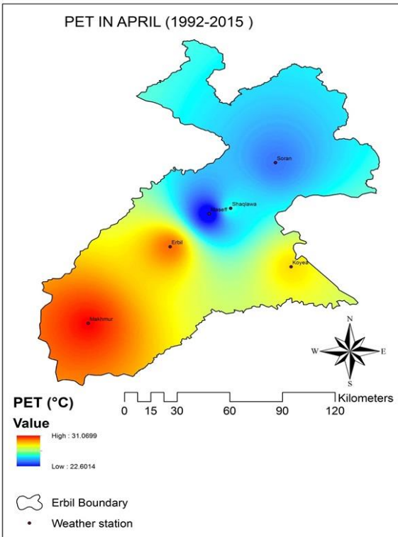
Figure 8. PET map of April
