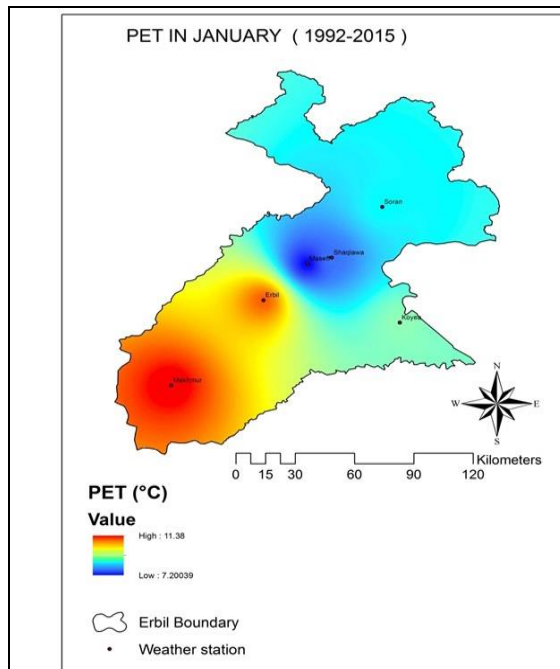
Figure 5. PET map of January
