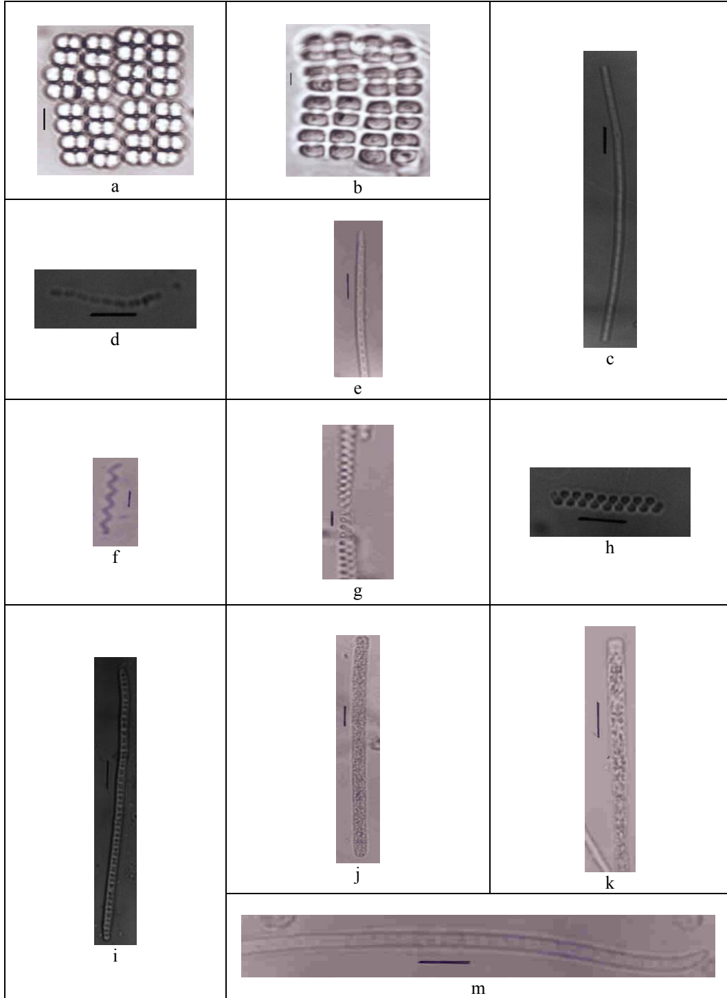
Şekil 3. a- Merismopedia elegans Lemmermann b- Merismopedia punctata Meyen c- Cylindrospermum stagnale (Kütz.) Born. et Flah. d- Anabaena circinealis var. macrospora (Witt.) De Toni e- Nostoc pruniforme Ag. f- Spirulina laxa G.M. Smith g- Spirulina major Kützing h- Spirulina princeps (West & West) G.S. West i- Oscillatoria amoena (Kuetz) Gomont j- Oscillatoria bornetii Zukal k- Oscillatoria prolifica (Grev) Gomont m- Oscillatoria splendida Graville (Ölçüler 10µm)
