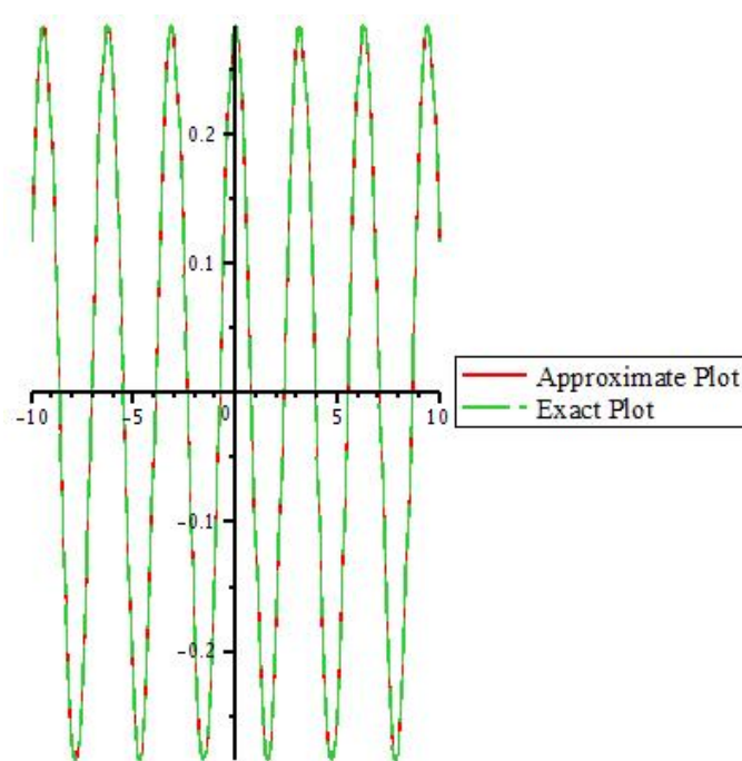
Figure 8: Graph of exact solution and 10th iteration of v by taking y=1 , a=2 , and b=5 .
