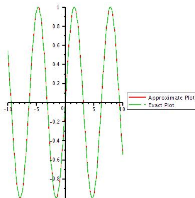
Figure 35: Graph of exact solution and 10th iteration of u by taking y=1 .
