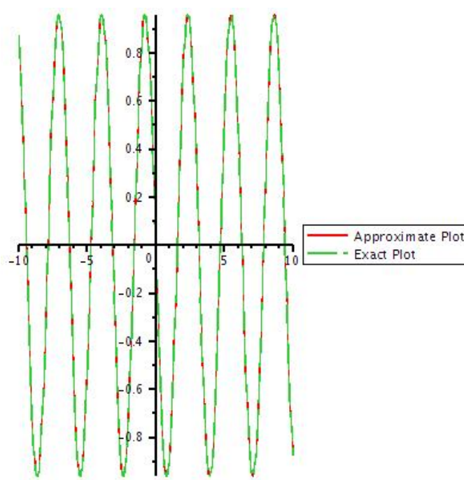
Figure 19: Graph of exact solution and 10th iteration of u by taking y=1 , a=2 , and b=5 .
