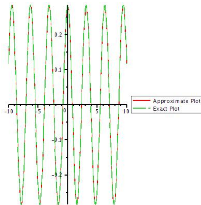
Figure 20: Graph of exact solution and 10th iteration of v by taking y=1 , a=2 , and b=5 .
