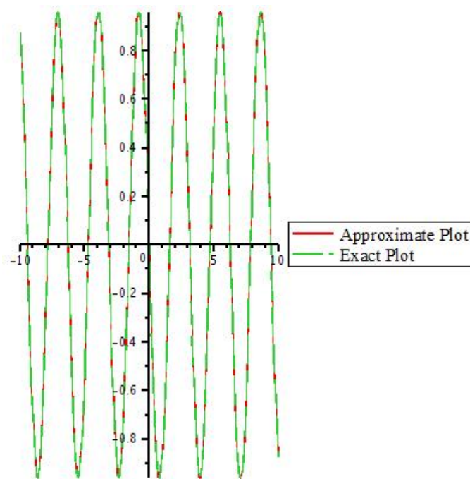
Figure 7: Graph of exact solution and 10th iteration of u by taking y=1 , a=2 , and b=5 .
