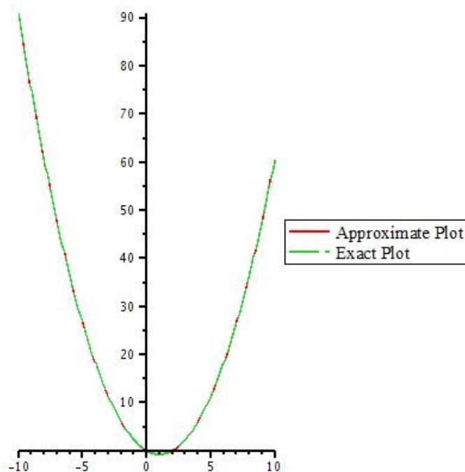
Figure 10: Graph of exact solution and 10th iteration of v by taking y=1 .
