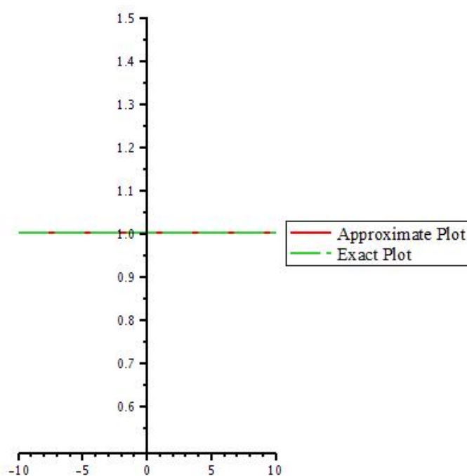
Figure 12: Graph of exact solution and 10th iteration of v by taking y=1 .
