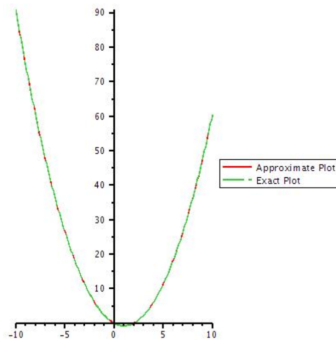
Figure 34: Graph of exact solution and 10th iteration of v by taking y=1 .
