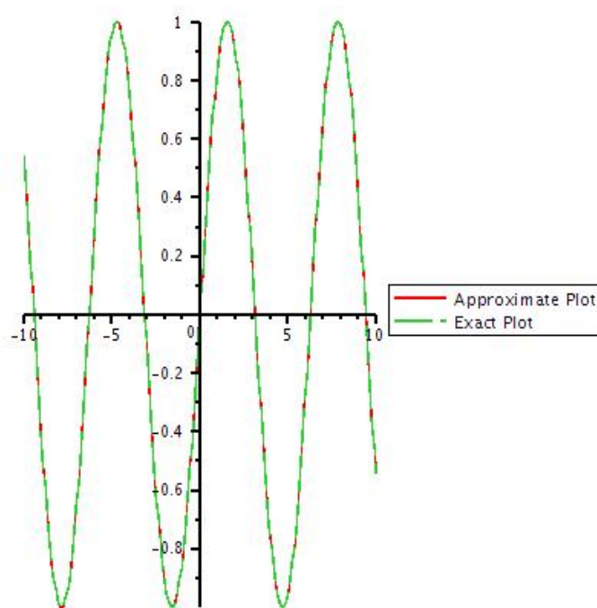
Figure 23: Graph of exact solution and 10th iteration of u by taking y=1 .
