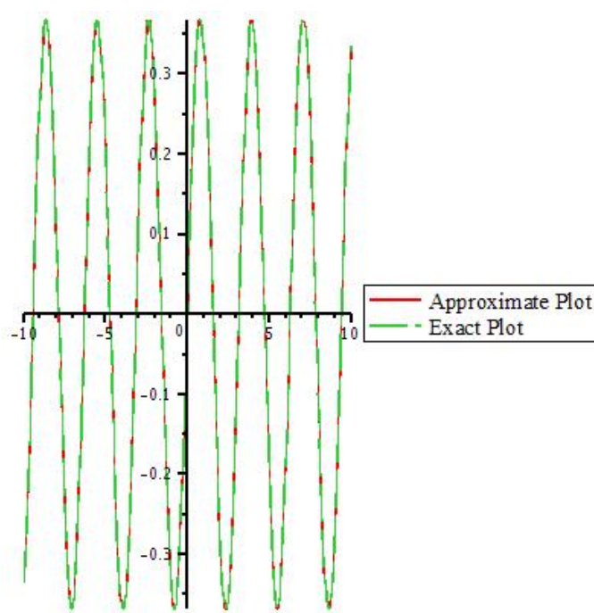
Figure 5: Graph of exact solution and 10th iteration of u by taking y=1 and a=2 .
