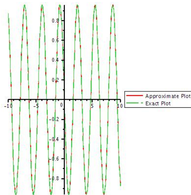
Figure 31: Graph of exact solution and 10th iteration of u by taking y=1 , a=2 , and b=5 .
