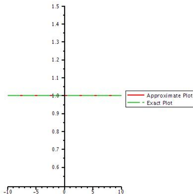
Figure 24: Graph of exact solution and 10th iteration of u by taking y=1 .
