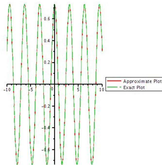
Figure 30: Graph of exact solution and 10th iteration of v by taking y=1 and a=2 .
