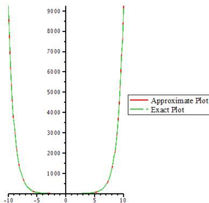
Figure 1: Graph of exact solution and 10th iteration of u by taking y=1 .
