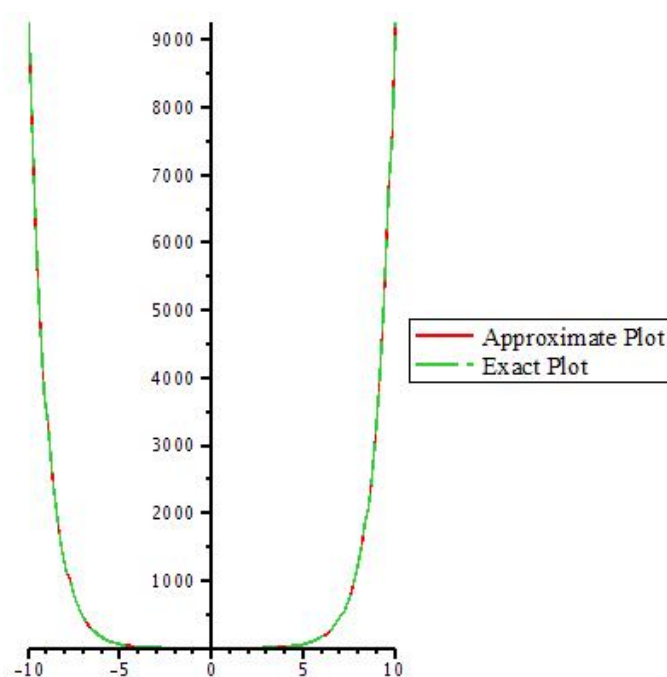
Figure 25: Graph of exact solution and 10th iteration of u by taking y=1 .
