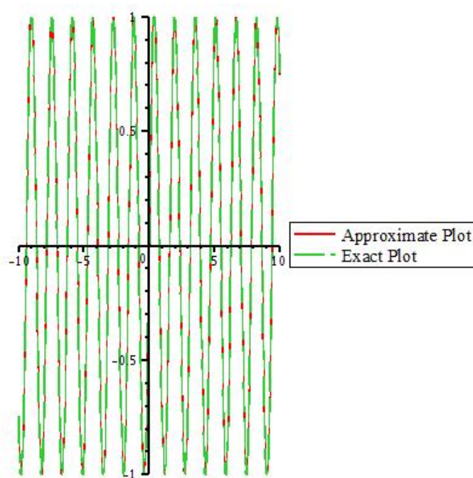
Figure 9: Graph of exact solution and 10th iteration of u by taking y=1 .
