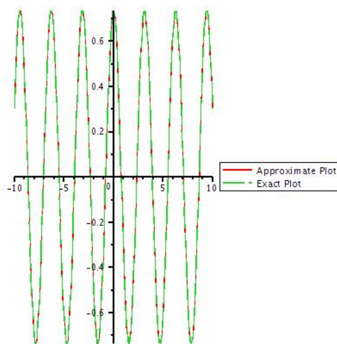
Figure 18: Graph of exact solution and 10th iteration of v by taking y=1 and a=2 .
