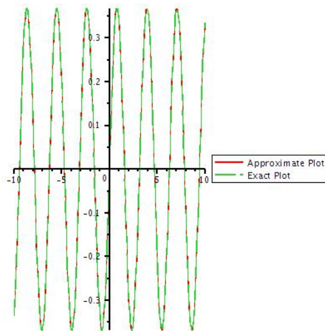
Figure 17: Graph of exact solution and 10th iteration of u by taking y=1 and a=2 .
