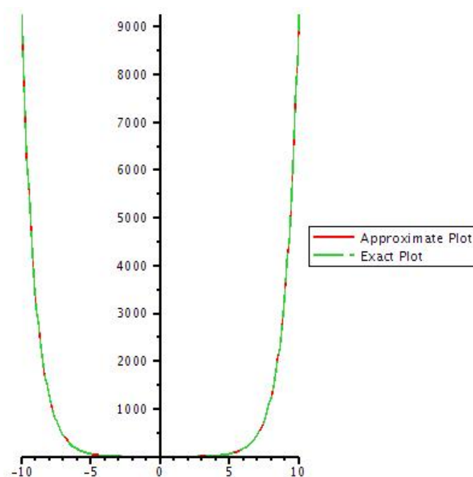
Figure 13: Graph of exact solution and 10th iteration of u by taking y=1 .
