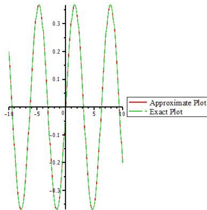
Figure 3: Graph of exact solution and 10th iteration of u by taking y=1 .
