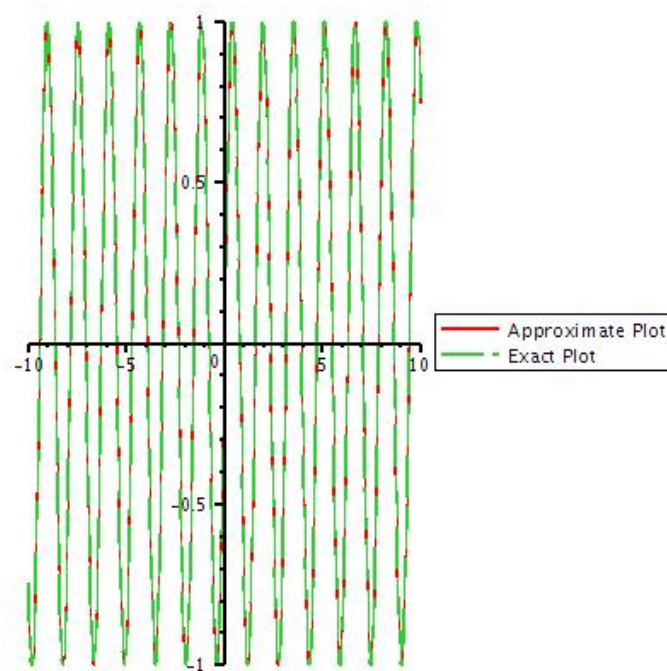
Figure 21: Graph of exact solution and 10th iteration of u by taking y=1 .
