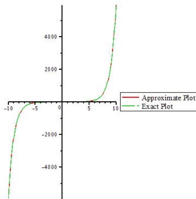
Figure 2: Graph of exact solution and 10th iteration of v by taking y=1 .
