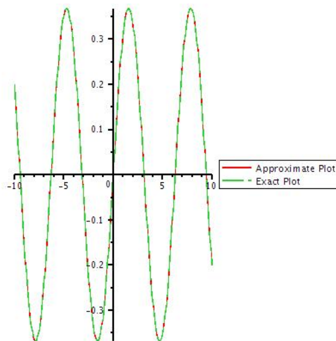
Figure 27: Graph of exact solution and 10th iteration of u by taking y=1 .
