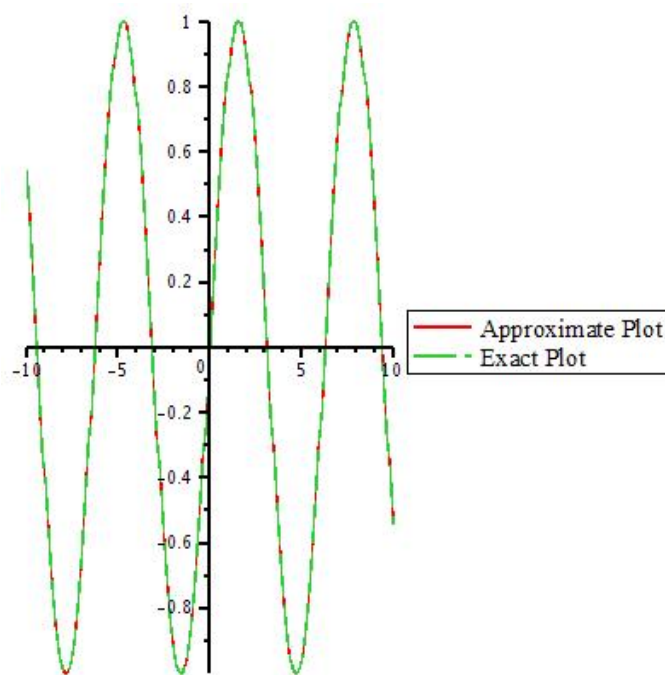
Figure 11: Graph of exact solution and 10th iteration of u by taking y=1 .
