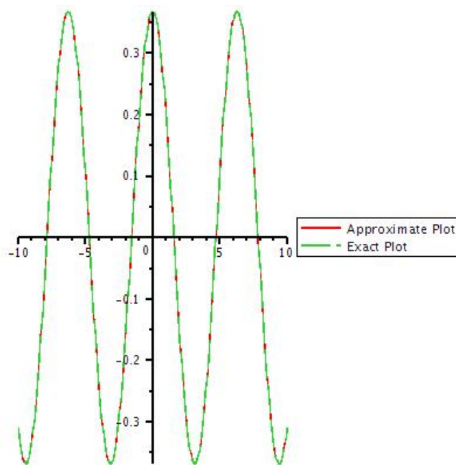
Figure 16: Graph of exact solution and 10th iteration of v by taking y=1 .
