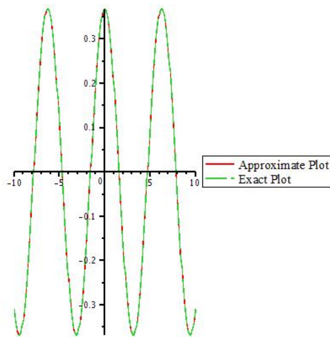
Figure 4: Graph of exact solution and 10th iteration of v by taking y=1 .
