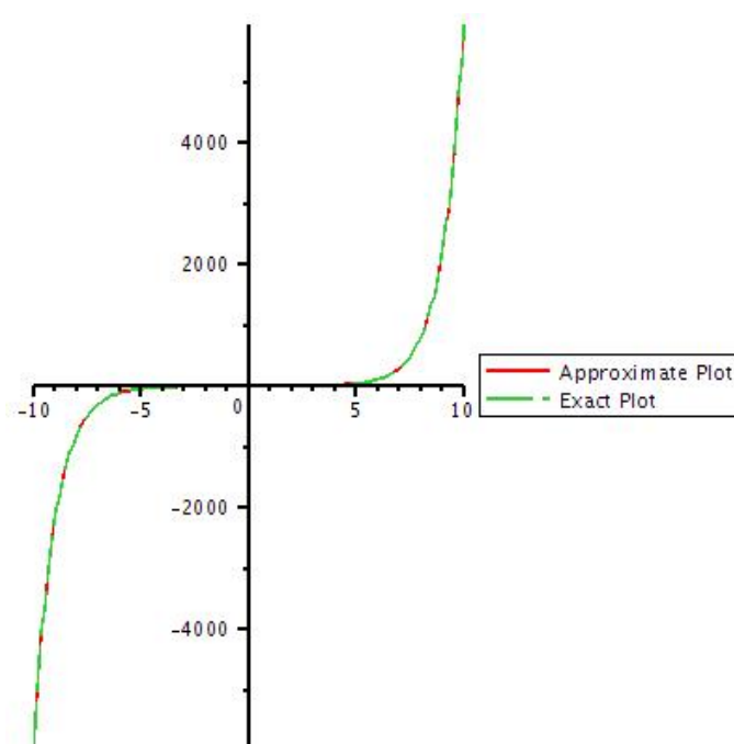
Figure 14: Graph of exact solution and 10th iteration of v by taking y=1 .
