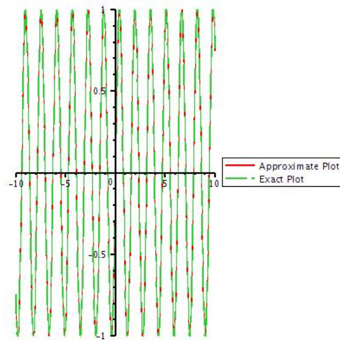
Figure 33: Graph of exact solution and 10th iteration of u by taking y=1 .
