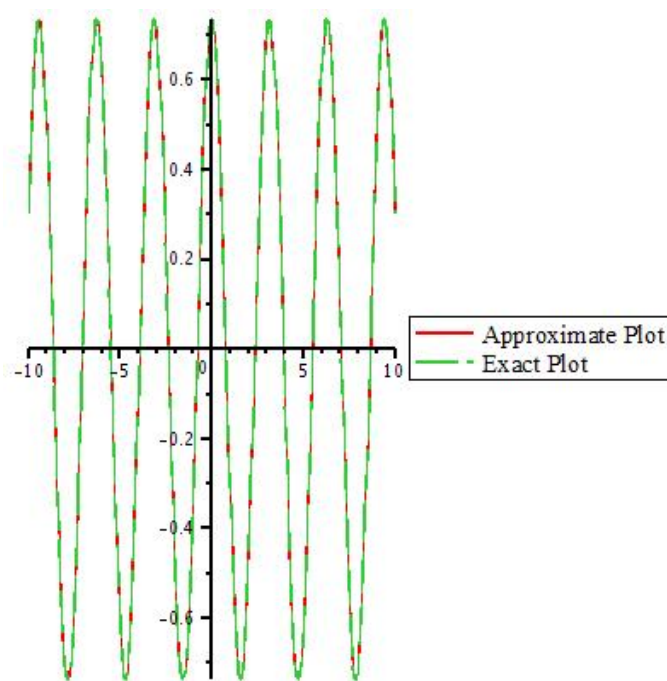
Figure 6: Graph of exact solution and 10th iteration of v by taking y=1 and a=2 .
