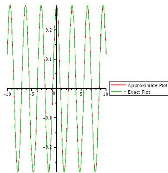
Figure 32: Graph of exact solution and 10th iteration of v by taking y=1 , a=2 , and b=5 .
