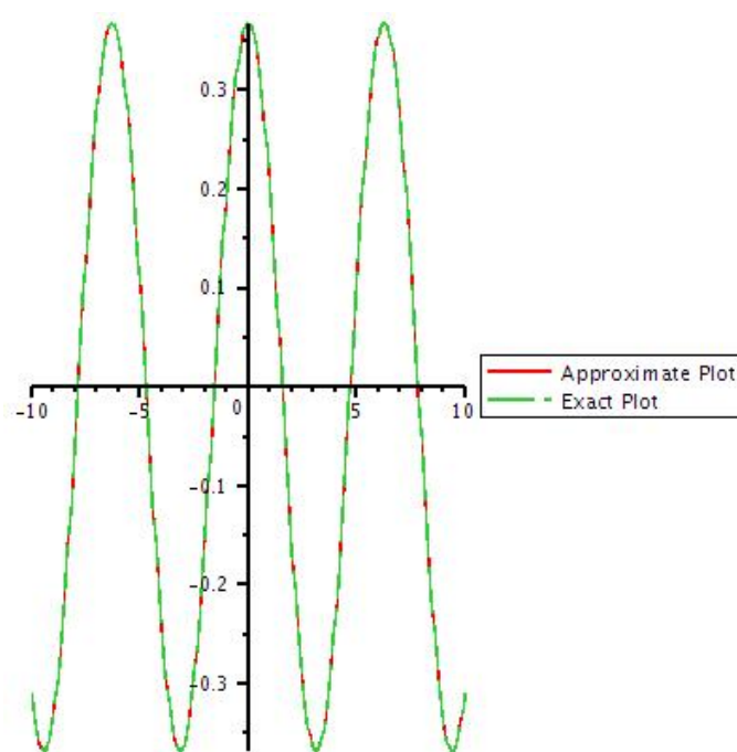
Figure 28: Graph of exact solution and 10th iteration of v by taking y=1 .
