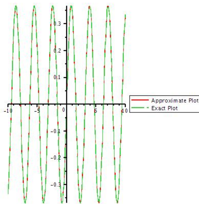
Figure 29: Graph of exact solution and 10th iteration of u by taking y=1 and a=2 .
