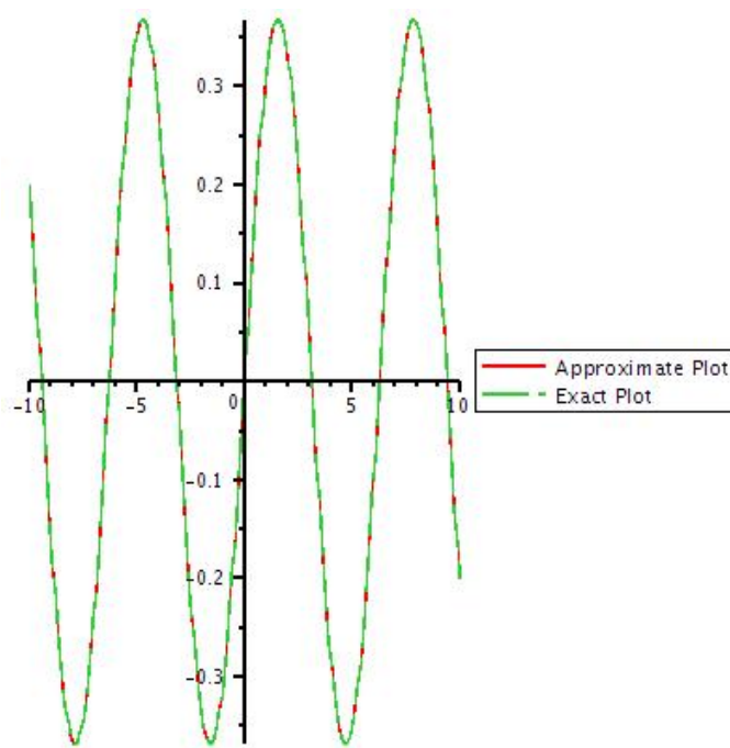
Figure 15: Graph of exact solution and 10th iteration of u by taking y=1 .
