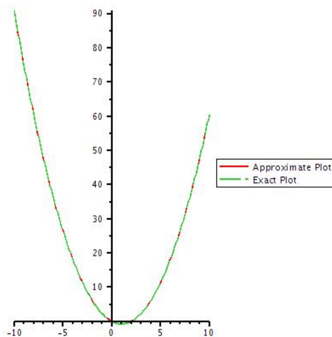
Figure 22: Graph of exact solution and 10th iteration of u by taking y=1 .
