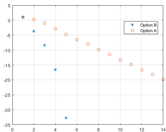
Figure 4: Graph of \log_{10} of the distance between two successive iterates (example 2).
