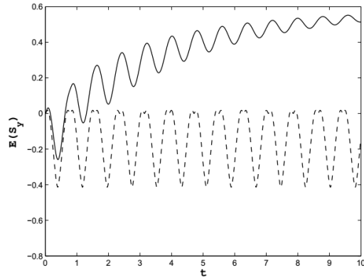
FIGURE 3. Entropy squeezing factor E(S_y) as a function of time t . n = 3 and k = 1 . The non-noisy case a = 0 and T \rightarrow \infty for dash line and a noisy case a = 0.4 and T = 1 for solid line.
