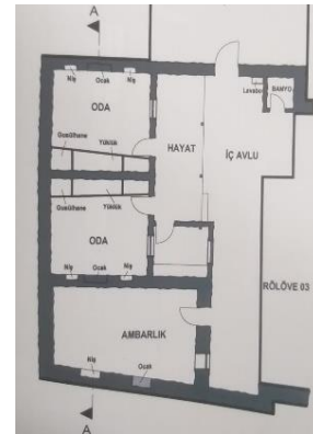
Plan 8. Zemin Kat Planı, H.Süleymaniye (İYTE, 2012c).
