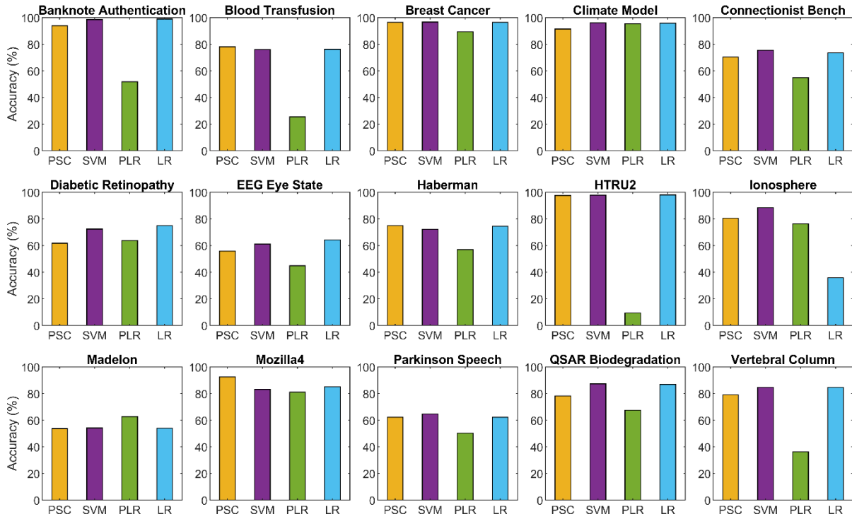
Figure 1. The comparative results of the algorithms relating to the classification accuracy.
