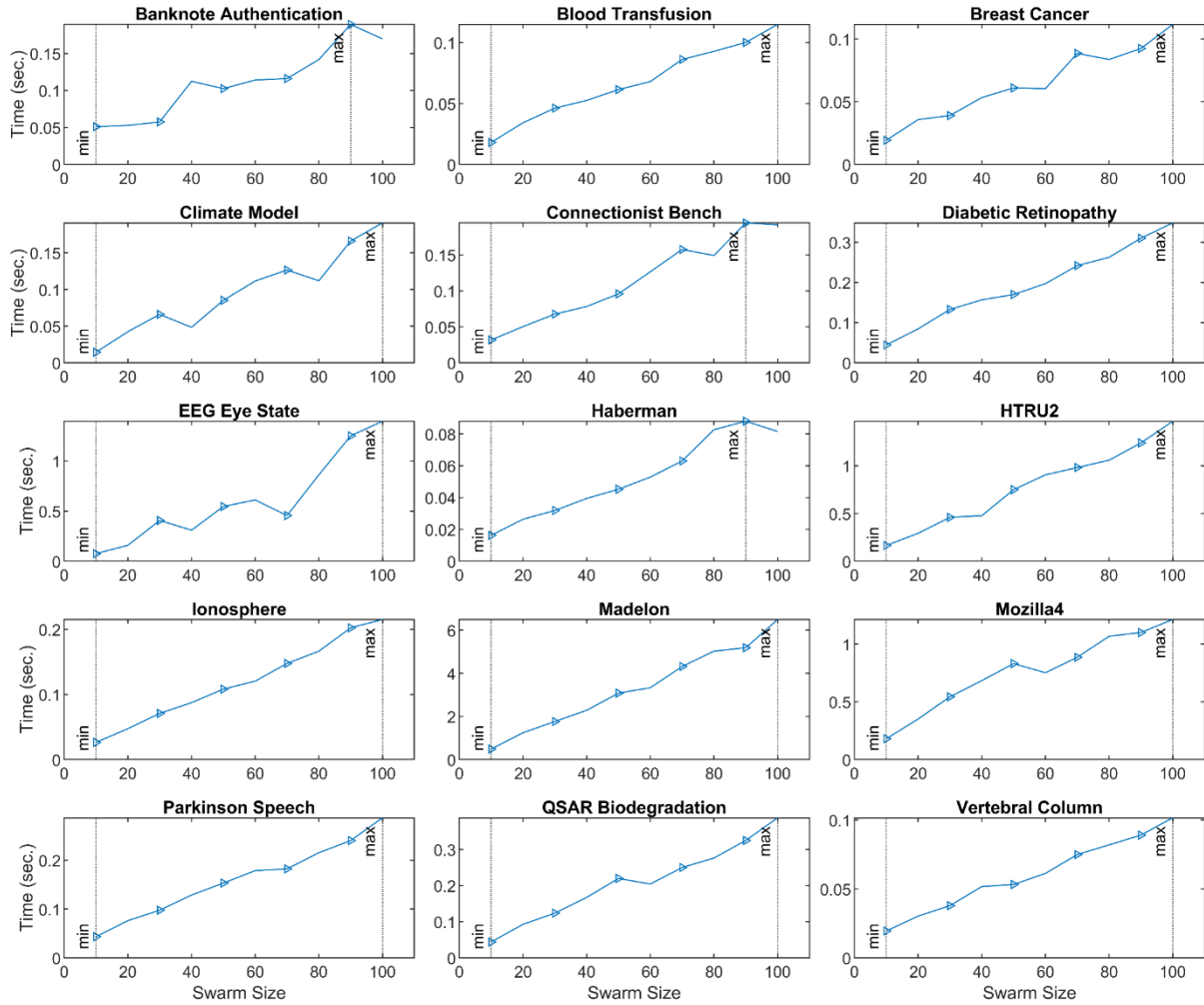
Figure 4. The change in the execution time according to the swarm size
