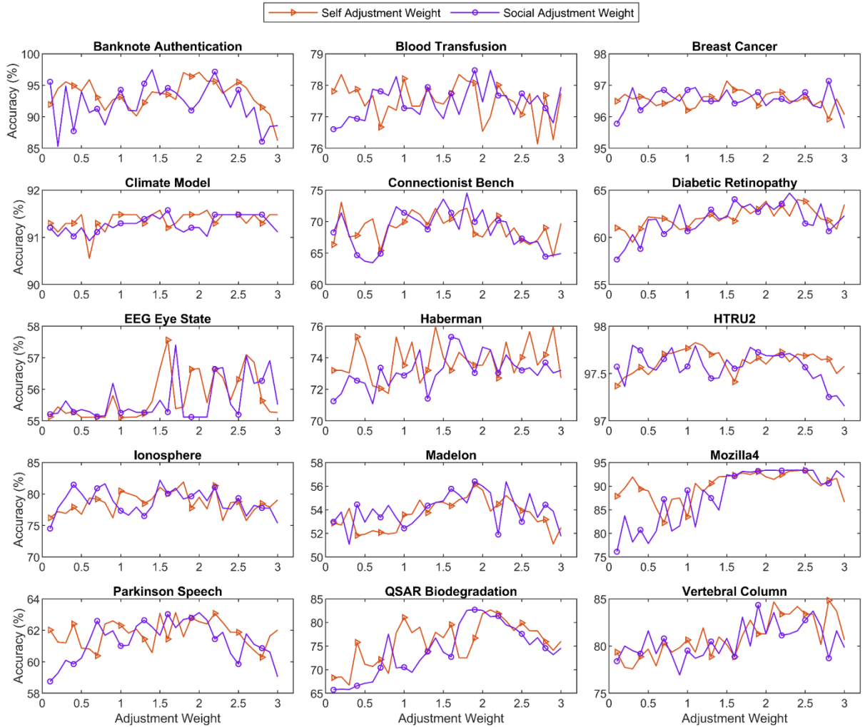
Figure 5. The change in the classification accuracy according to the adjustment weight
