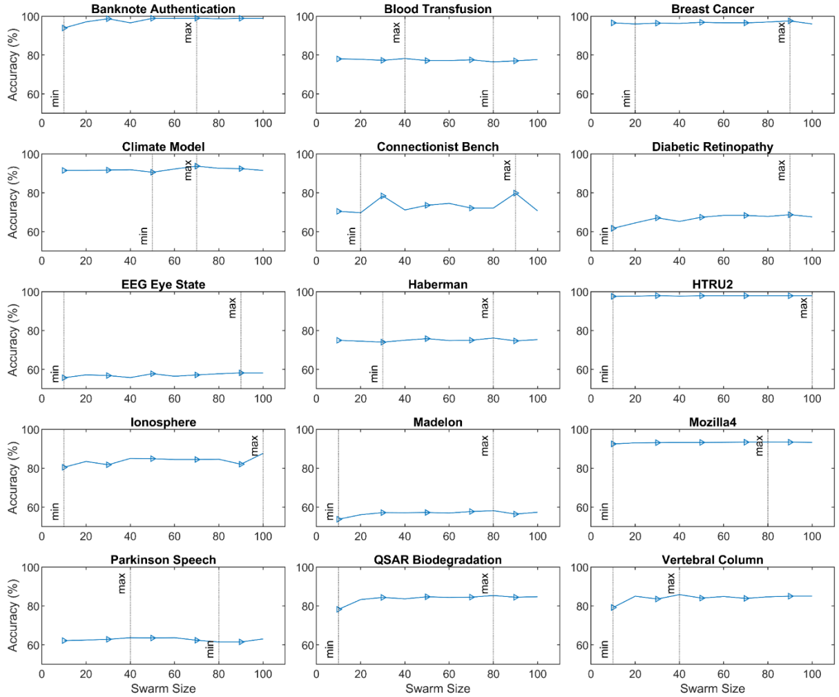
Figure 3. The change in the accuracy rate according to the swarm size
