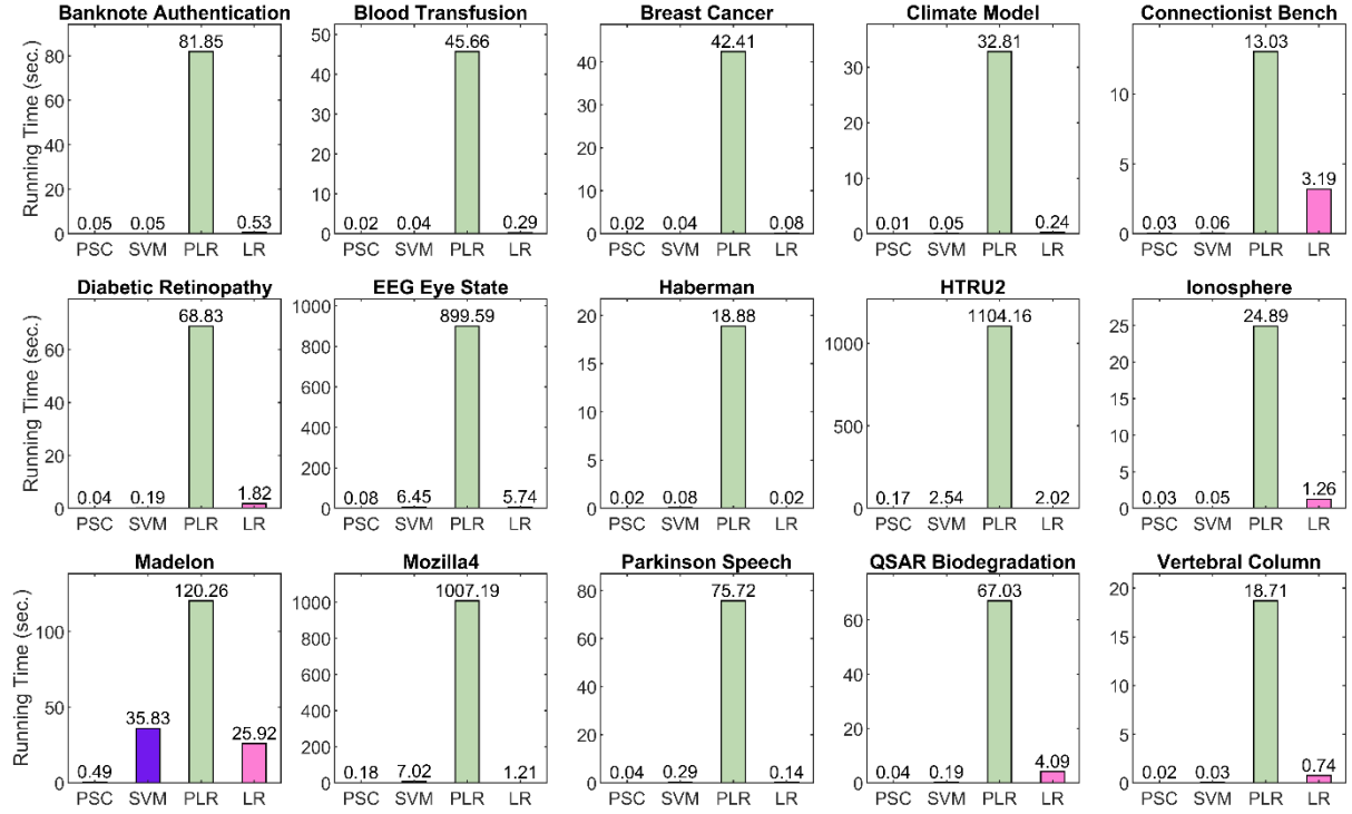
Figure 2. The comparative results of the classifiers with respect to the execution time
