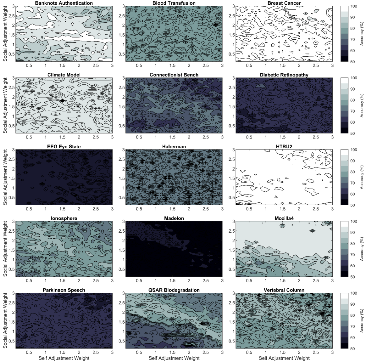
Figure 6. The variation in the classification accuracy with both adjustment weights
