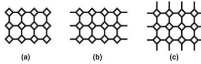
FIGURE 1. (a) 2D -lattice of TUC_4C_8[p, q] ; (b) nanotubes of TUC_4C_8[p, q] ; (c) nanotoruses of TUC_4C_8[p, q] .
