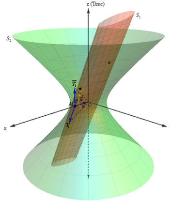
FIGURE 2. A Lorentzian Unit Sphere S_1^2 Rolling on a Timelike Cylinder with radius \frac{3}{4}
