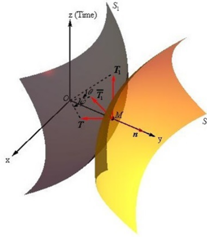
FIGURE 1. The timelike surface S_2 rolling on the timelike surface S_1 in the direction of timelike unit tangent vector T
