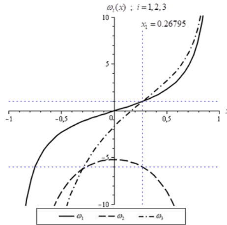
FIGURE 3. The angular velocity components with respect to x = \tanh((\varphi + \theta)/2)
