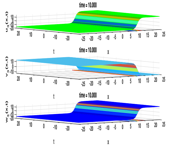
Figure 3 Traveling wave profile for the solution (25)
