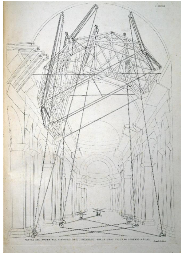
Figure 8. Pizzagalli & Aluisetti 1827, pl. XXVIII, showing the installation of the 18 th century scaffolding by Pietro Albertini in the nave of St. Peter's, from Zabaglia 1824, pl. LX (here in Fig. 4).
