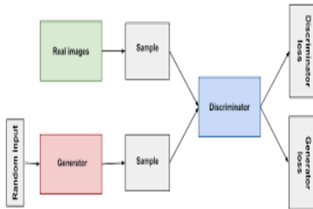
Fig. 1 GAN Algorithm
