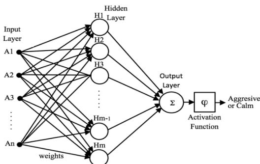
Figure 5. Designed ANN
