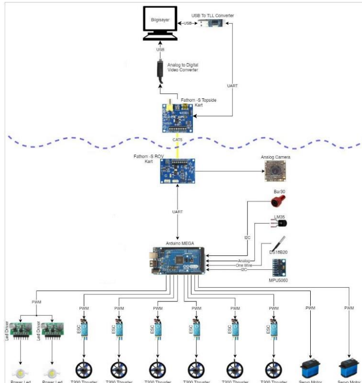
Figure 3. Communication infrastructure of the vehicle
