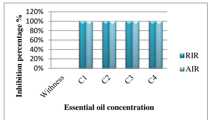
Figure 2. Inhibition of RIR and AIR recorded for Wheat seeds treated with F.vulgare oil.
