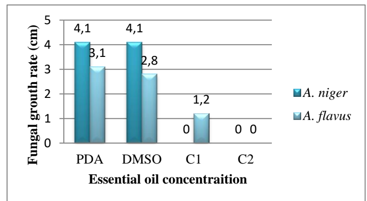
Figure 4. Mycelial diameter growth under the effect of F. vulgare oil
