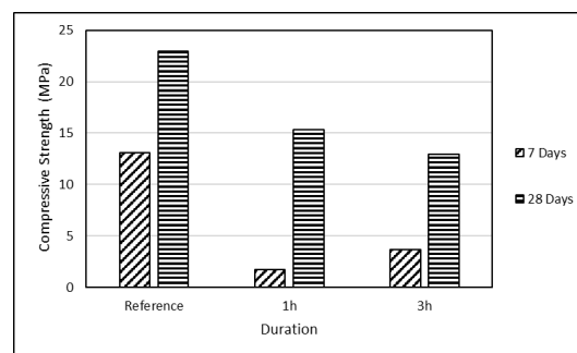
Fig. 5 The compressive strength of geopolymer pastes aged for 7 and 28 days
