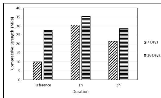
Fig. 4 The compressive strength of cement mortars aged for 7 and 28 days
