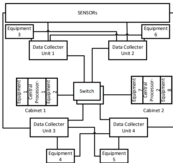
Figure 8 Distributed Integrated Modular Architecture
