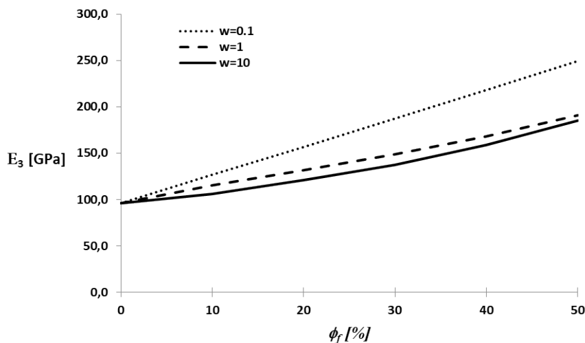
Figure 5. Modulus E_3 versus the fiber volume fraction for various shape ratios ( w = 0.1, 1 and 10 ). Mori-Tanaka scheme
