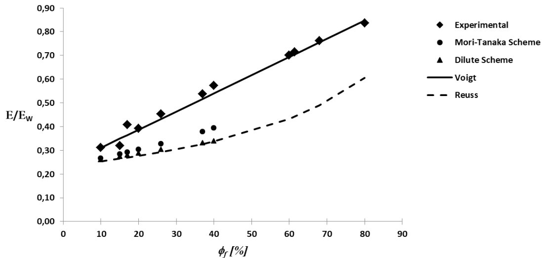
Figure 1. Variation of the normalized Young's modulus E/E_w ( E_w is the Young's modulus of Tungsten fiber) as a function of the volume fraction of tungsten fiber: Comparison between experimental data [12, 13, 22-24] and homogenization schemes.
