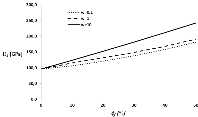
Figure 4. Modulus E_1 versus the fiber volume fraction for various shape ratios ( w = 0.1, 1 and 10 ). Mori-Tanaka scheme
