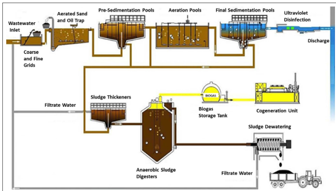
Figure 5. Classic domestic wastewater treatment plant model [15].
