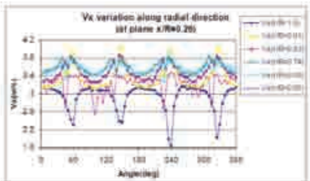
Figure 24 The axial component V_x (including V_\theta ) in the propeller race
