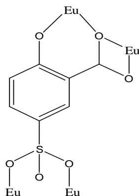
Scheme 1. The coordination mode of ssa ligand of complex ( 1 ).
