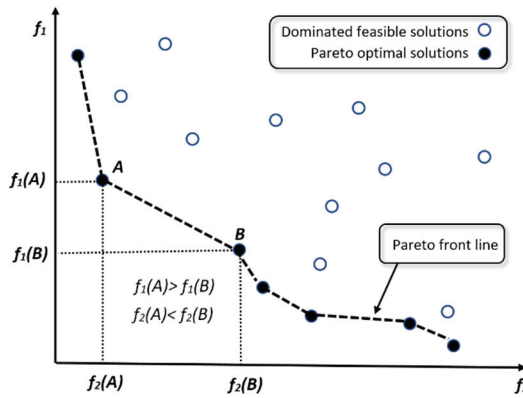
Figure 3. Feasible solutions of a multi-objective problem with two conflicting objective functions
