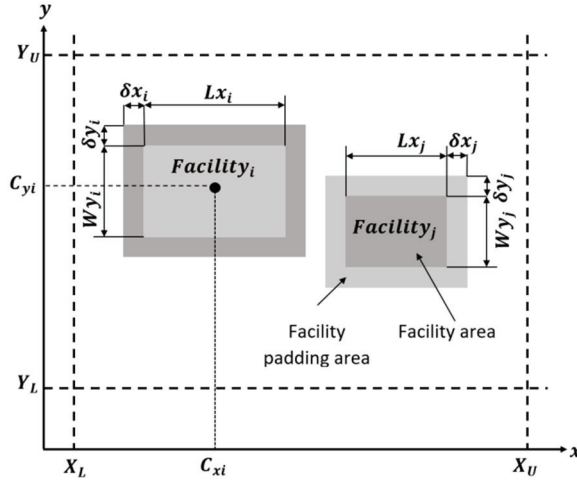
Figure 2. Boundary and overlap constraints
