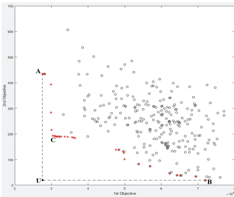
Figure 11. Pareto optimal solutions (Results of the case study)
